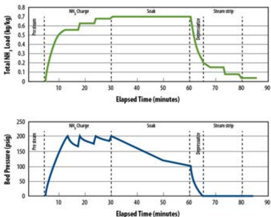
Figure 4–2. Ammonia loading and bed pressure during AFEX® treatment as a function of time.
