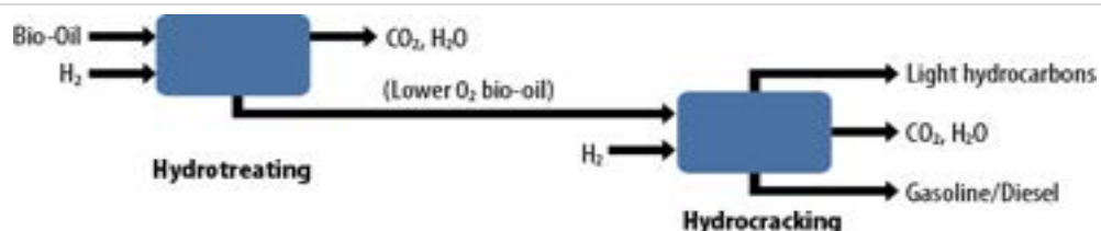
Figure 6–10. Bio-oil stabilization and upgrading
