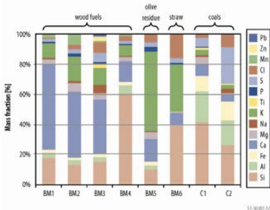
Figure 4–4. Ash elements in biomass versus coal.
