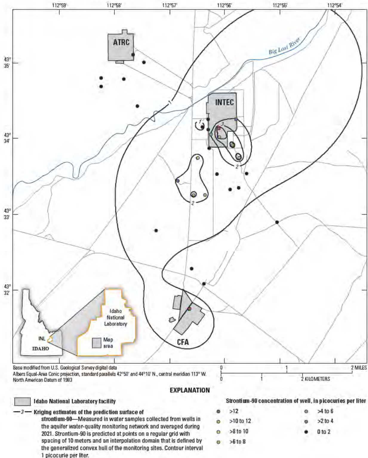
Figure 6-6. Distribution of ^{90}\text{Sr} (pCi/L) in the eastern Snake River Plain Aquifer onsite in 2021 (from Treinen et al. 2024).
