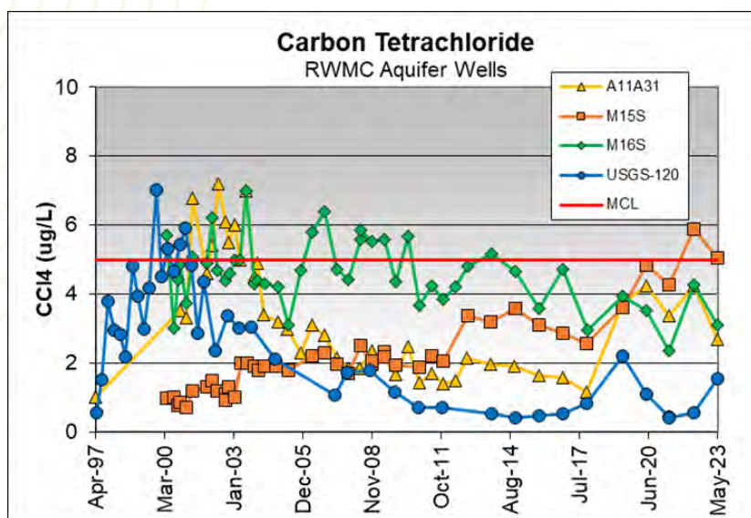
Figure 6-16. Carbon tetrachloride (CCl 4 ) concentration trends in RWMC aquifer Wells A11A31, M15S, M16S, and USGS-120.
