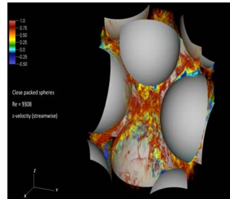
Turbulent Heat Flux – Nek5000/BISON
