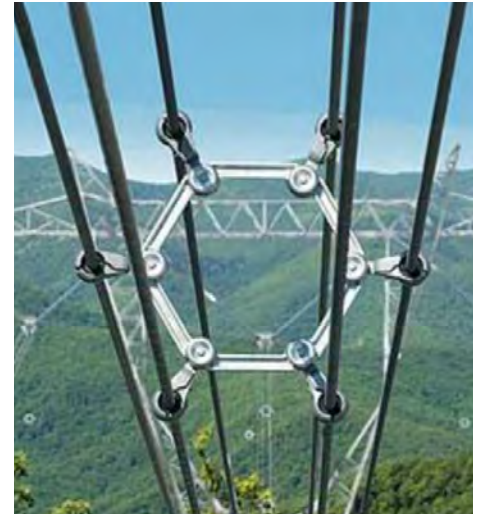
Figure 2-16. Example of bundled conductor to reduce corona effect on transmission power lines.
