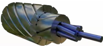
Figure A-56. ACSS/TW conductor.
