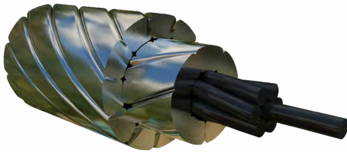
Figure 2-8. C7 conductor.
