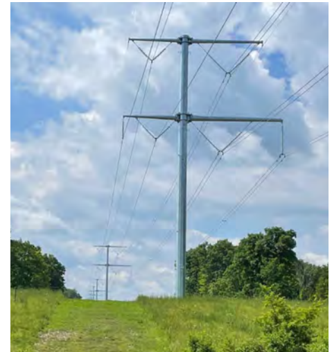
Figure 2-17. A double circuit rebuild for the New Your Energy Solution project with the 115 kV circuit on the left side of the tower and the 345 kV circuit on the right side of the tower.
