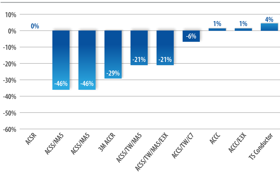
Figure 2-14. Efficiency change at the maximum continuous temperature of various conductors with respect to percentage deviation from ACSR's efficiency at max continuous operating temperature.
