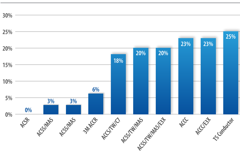
Figure 2-13. Efficiency of conductors at 20°C vs. ACSR.
