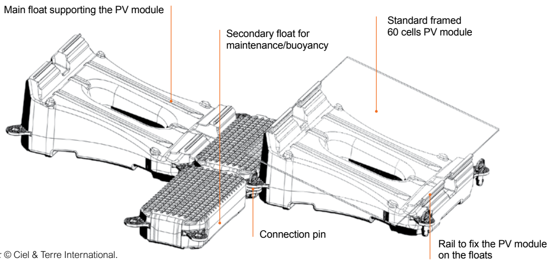
FIGURE 2.3. Components of floats from Ciel & Terre International
