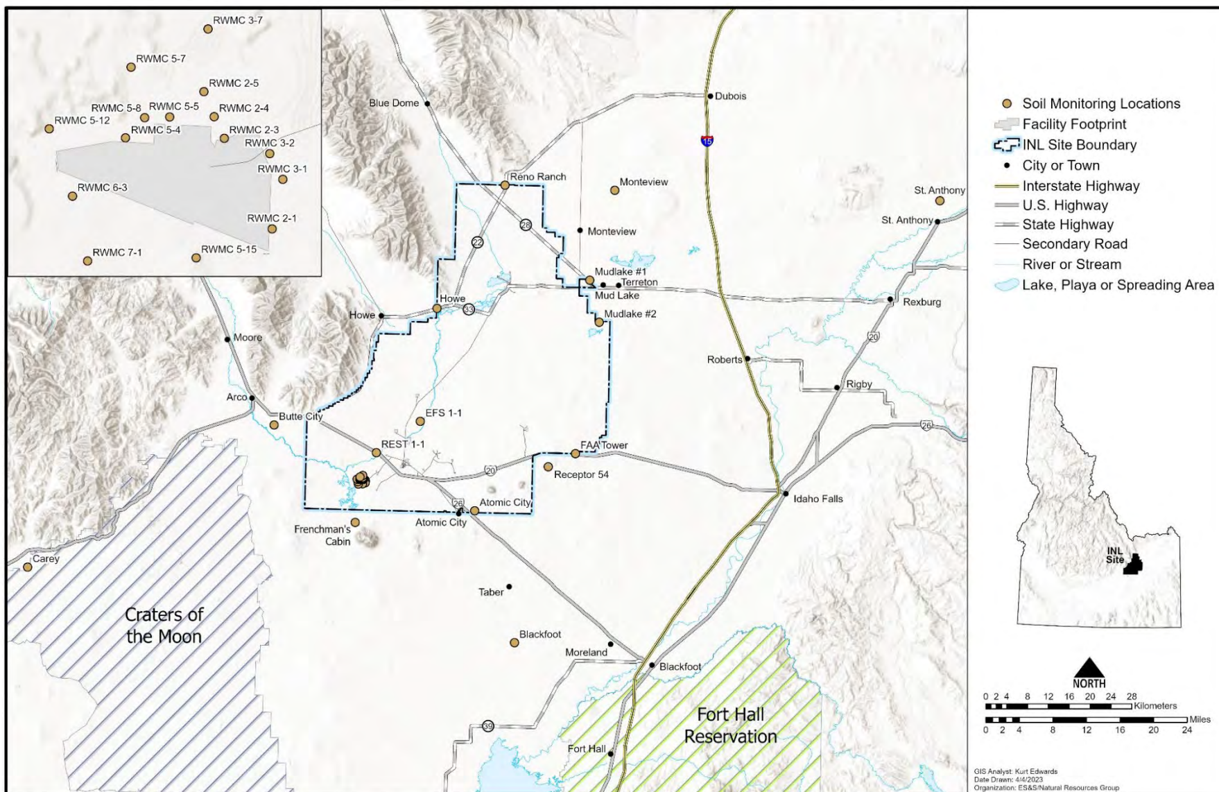
Figure 7-3. Soil sampling locations in 2022.
