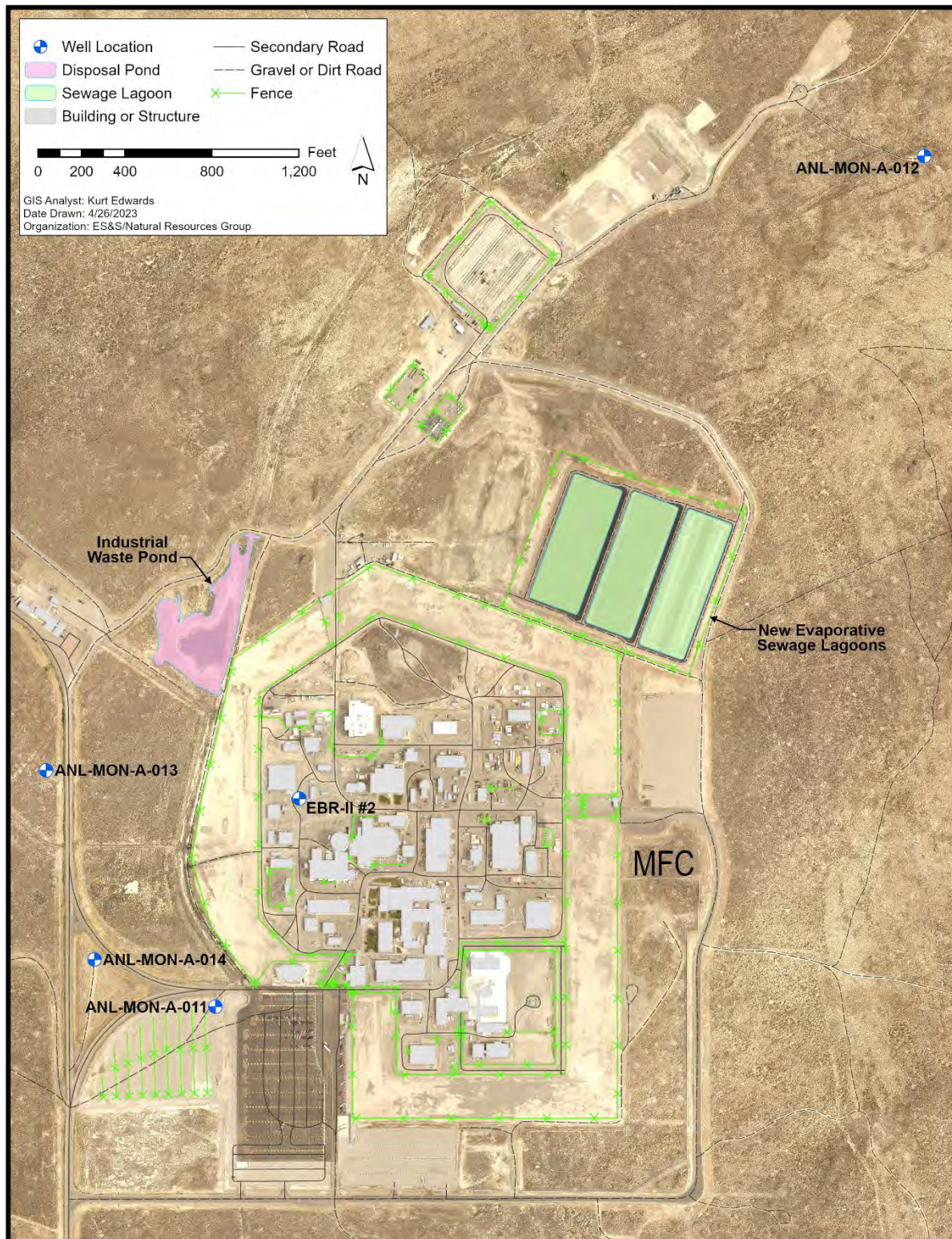
Figure 6-19. Locations of WAG 9 wells sampled in 2022.
