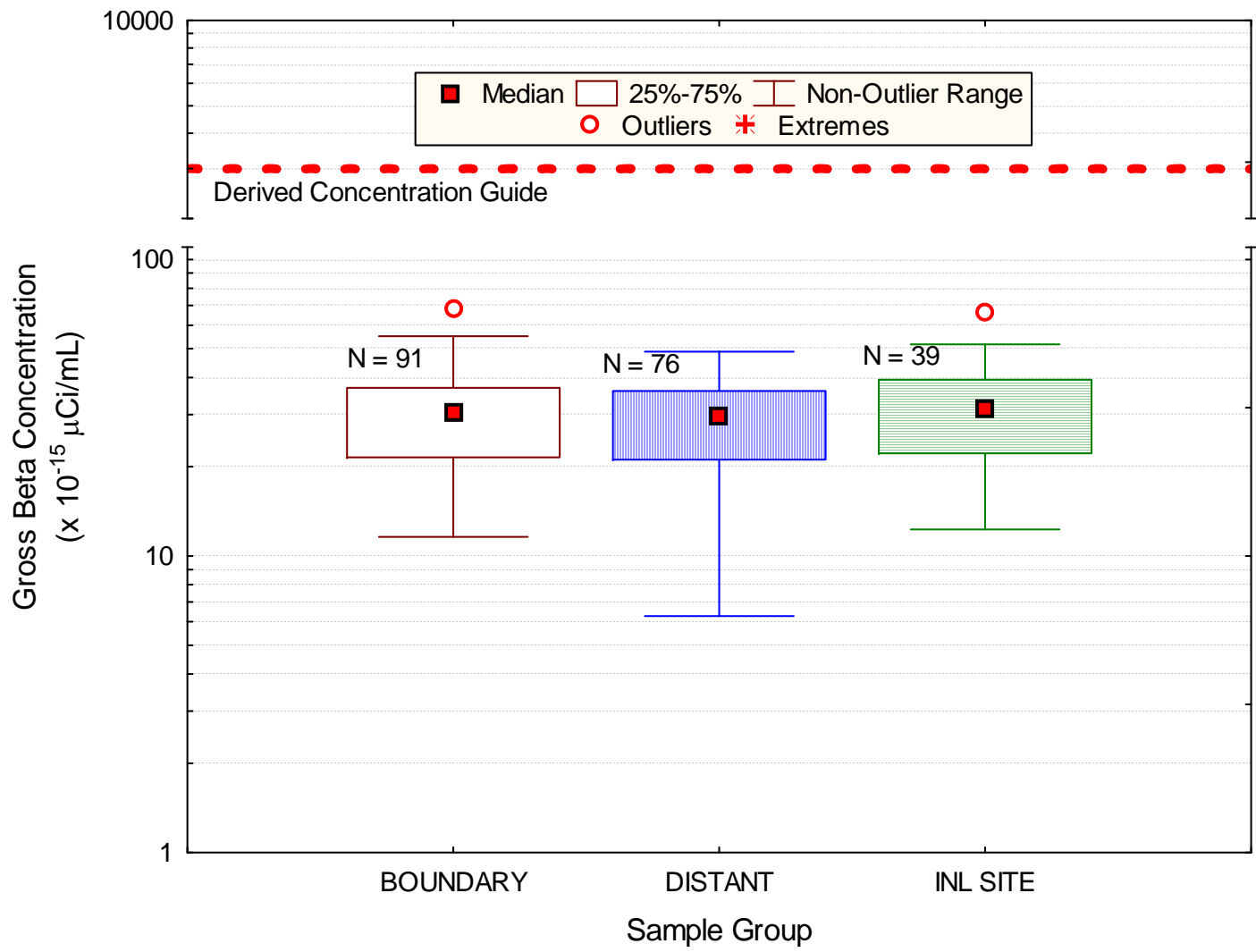
Figure 7. Gross beta concentrations in air at ESER INL Site, Boundary and Distant locations for the first quarter of 2010.
