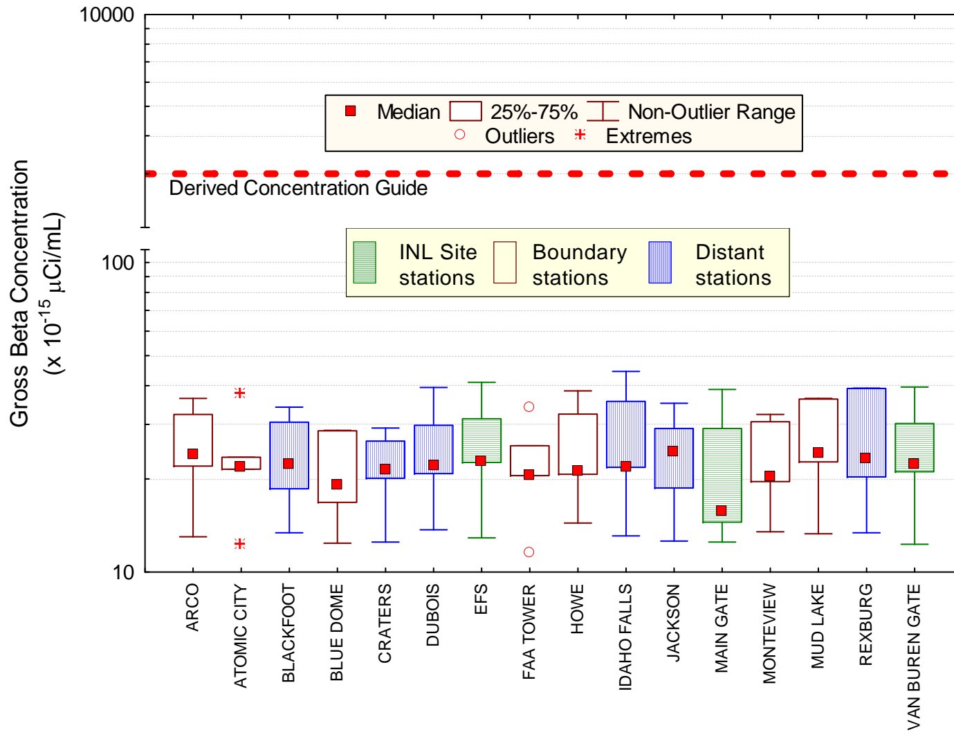
Figure 10. March gross beta concentrations in air at ESER INL Site, Boundary and Distant locations. Number of samples (N) = 5 at each location.
