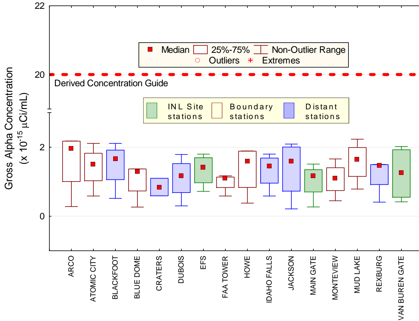
Figure 4. January gross alpha concentrations in air at ESER INL Site, Boundary and Distant locations. Number of samples (N) = 4 at each location, except Craters (N = 3).
