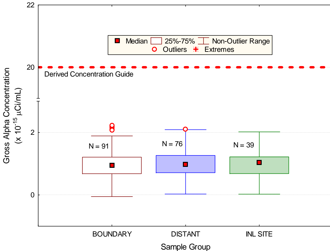
Figure 3. Gross alpha concentrations in air at ESER INL Site, Boundary and Distant locations for the first quarter of 2010.
