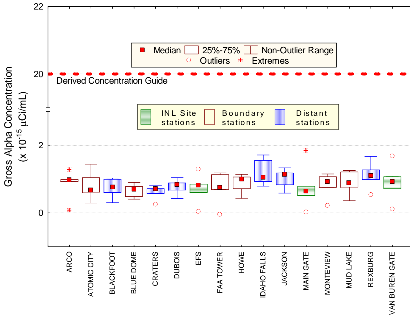
Figure 6. March gross alpha concentrations in air at ESER INL Site, Boundary and Distant locations. Number of samples (N) = 5 at each location.
