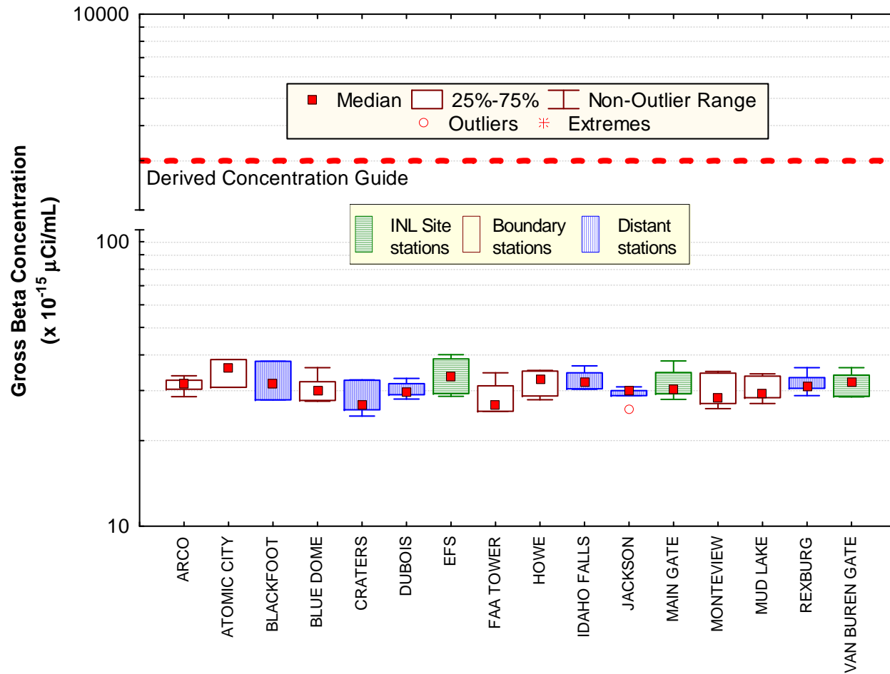
Figure 8. July gross beta concentrations in air at ESER INL Site, Boundary and Distant locations. Number of samples (N) = 5 at each location, except FAA Tower (N = 4), Atomic City and Blackfoot (N = 3).
