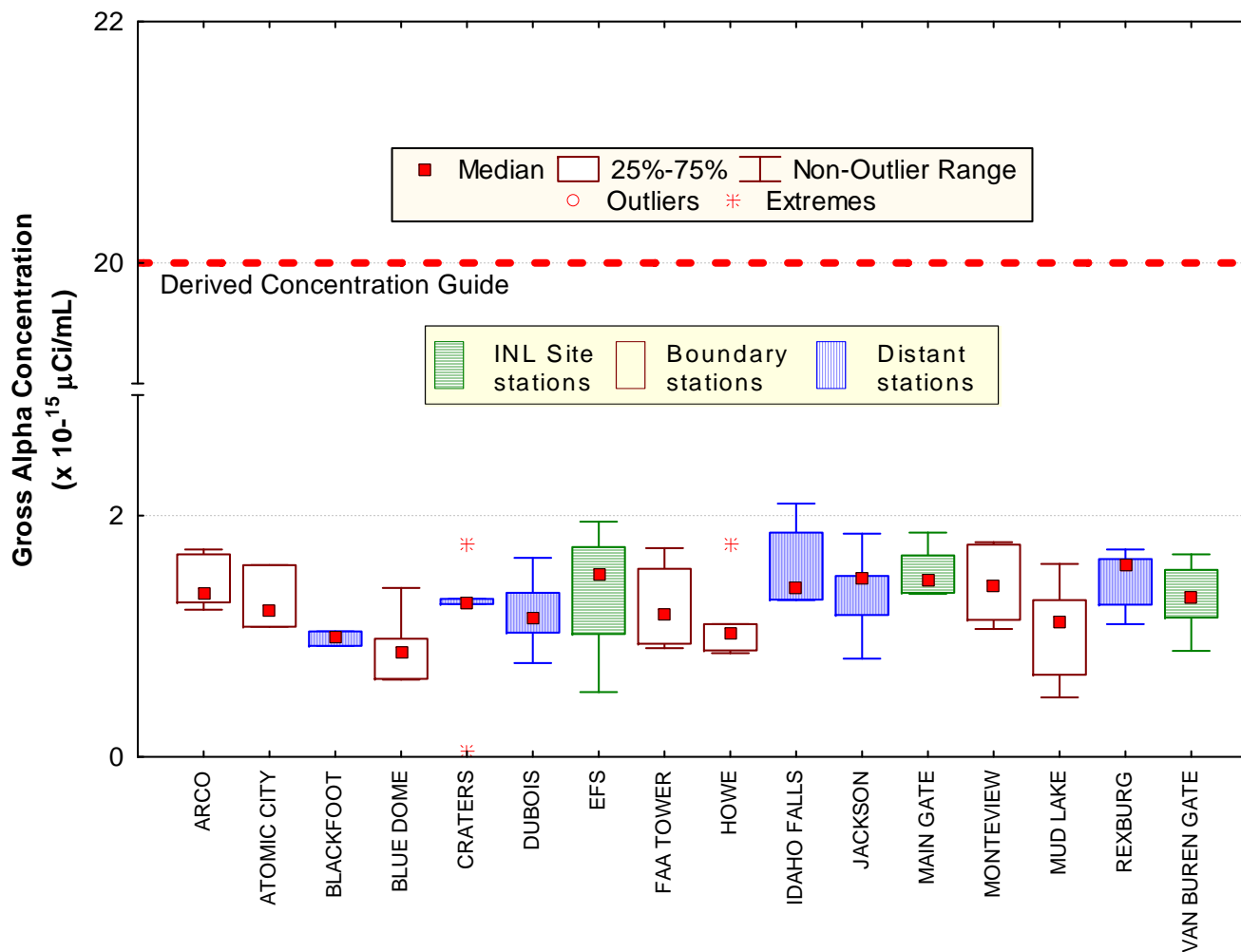
Figure 4. July gross alpha concentrations in air at ESER INL Site, Boundary and Distant locations. Number of samples (N) = 5 at each location, except EFS, FAA Tower (N = 4), Atomic City and Blackfoot (N = 3).
