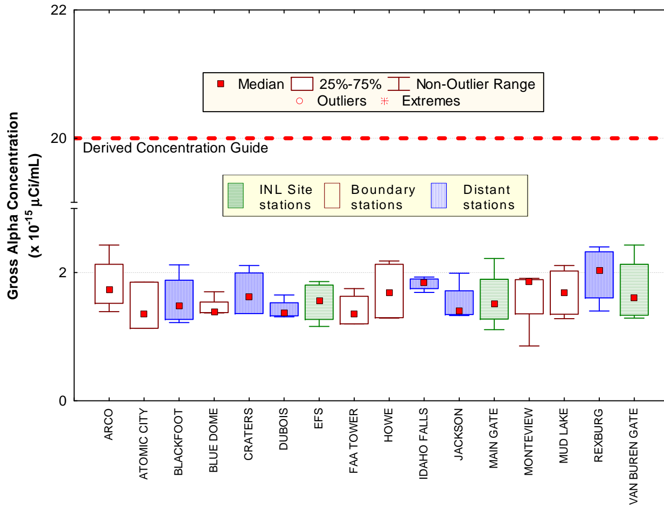
Figure 5. August gross alpha concentrations in air at ESER INL Site, Boundary and Distant locations. Number of samples (N) = 4 at each location, except Atomic City (N = 3).
