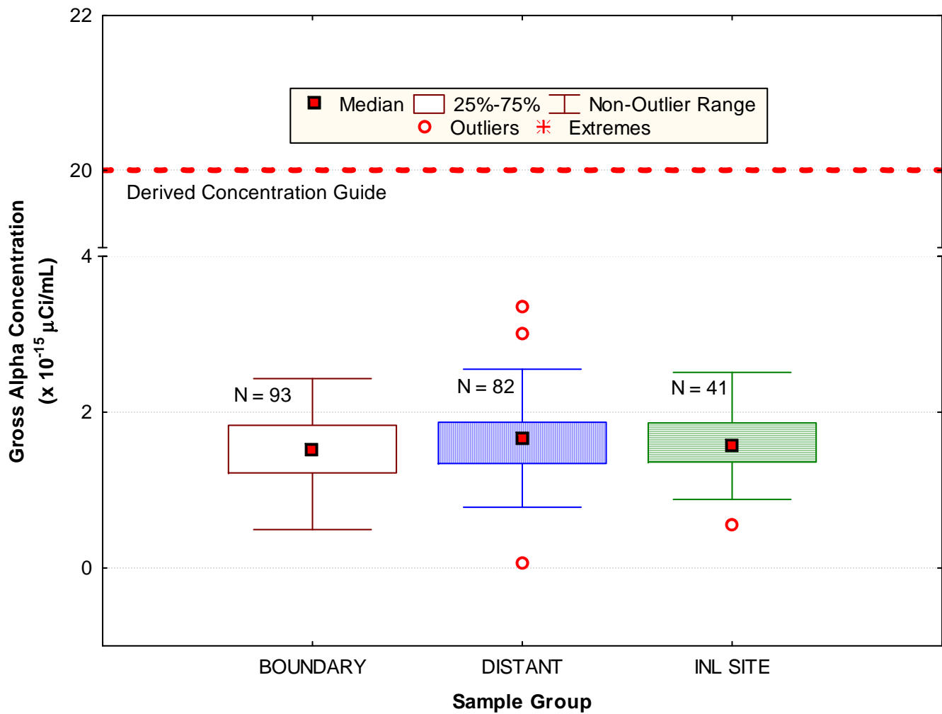
Figure 3. Gross alpha concentrations in air at ESER INL Site, Boundary and Distant locations for the third quarter of 2009.
