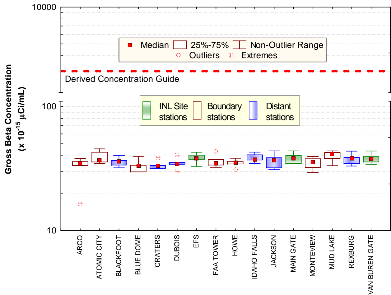
Figure 10. September gross beta concentrations in air at ESER INL Site, Boundary and Distant locations. Number of samples (N) = 5 at each location, except Monteview (N = 4).
