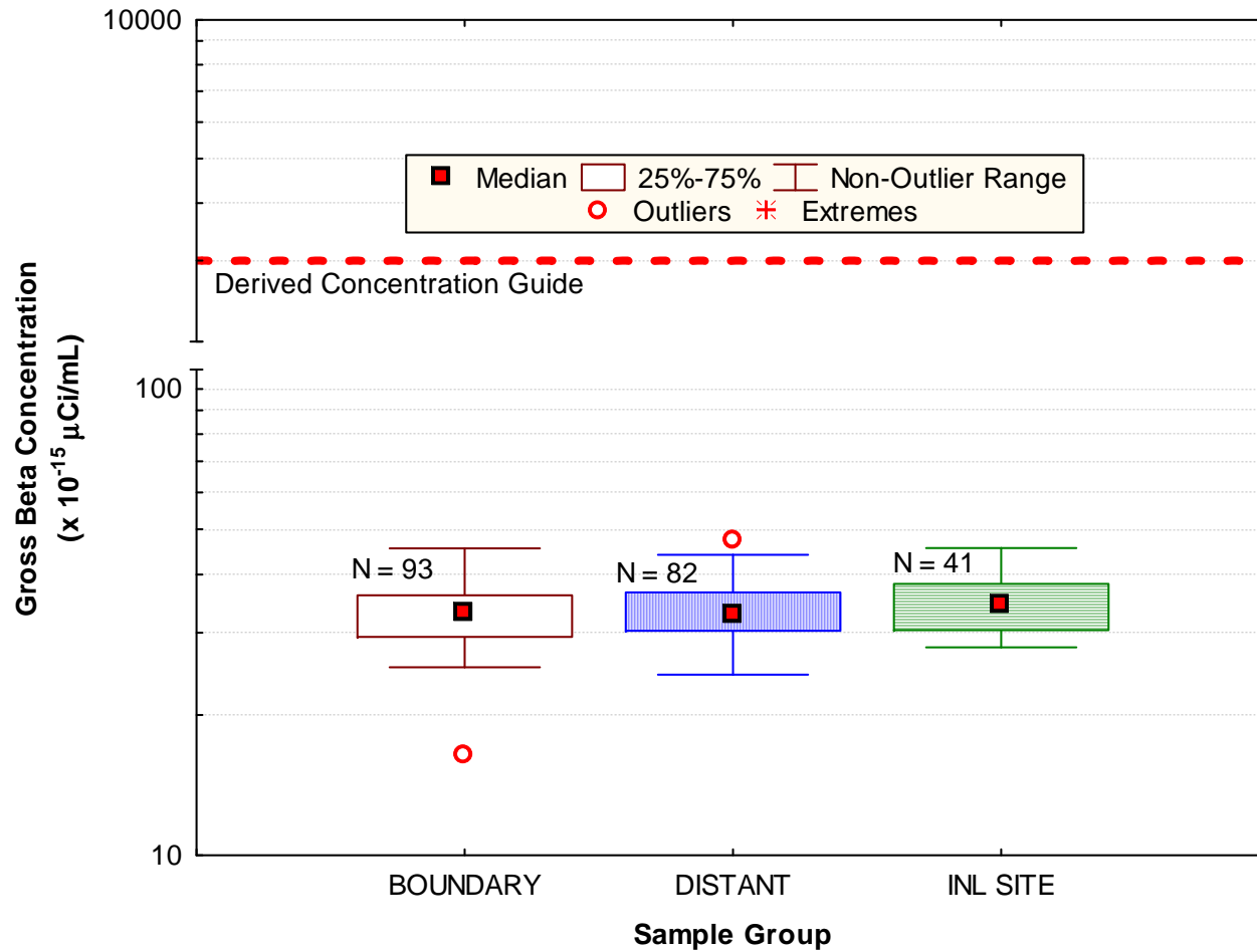
Figure 7. Gross beta concentrations in air at ESER INL Site, Boundary and Distant locations for the third quarter of 2009.
