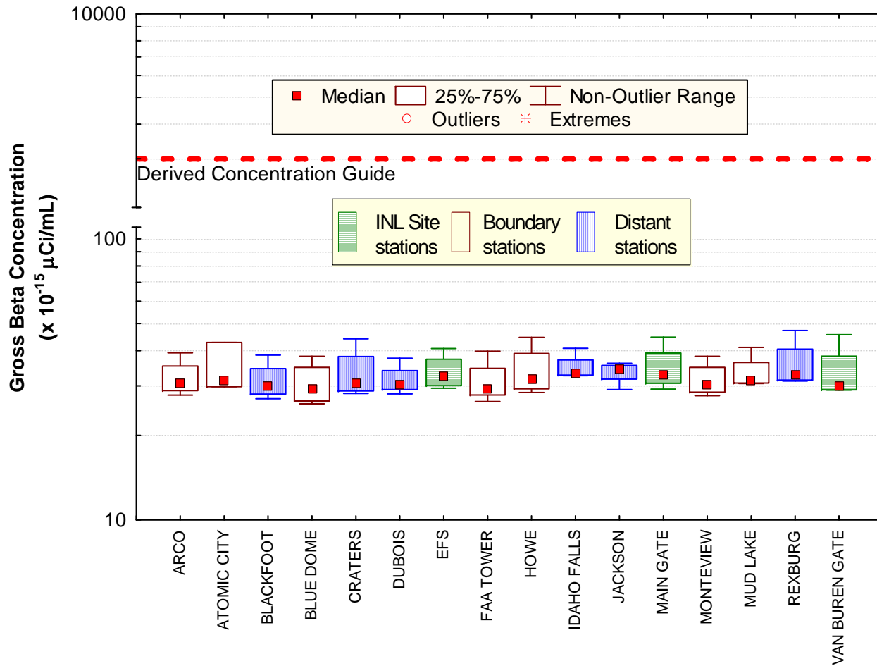
Figure 9. August gross beta concentrations in air at ESER INL Site, Boundary and Distant locations. Number of samples (N) = 4 at each location, except Atomic City (N = 3).
