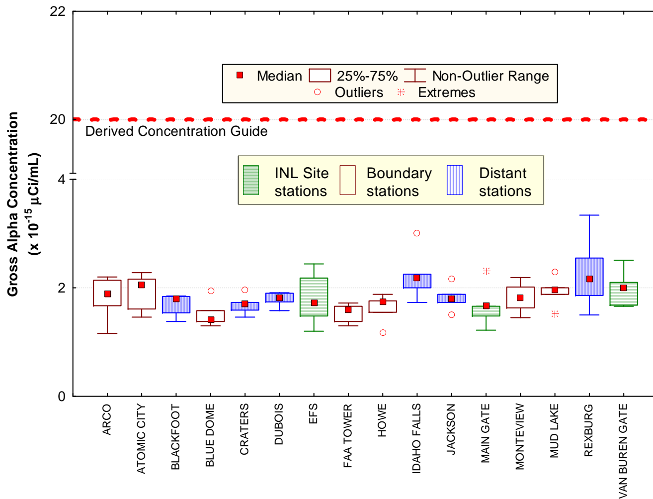
Figure 6. September gross alpha concentrations in air at ESER INL Site, Boundary and Distant locations. Number of samples (N) = 5 at each location, except Monteview (N = 4).
