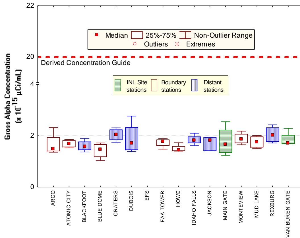
Figure 5. August gross alpha concentrations in air at ESER INL Site, Boundary and Distant locations. Number of samples (N) = 4 at each location, except Jackson (N = 3) and EFS (N = 0).
