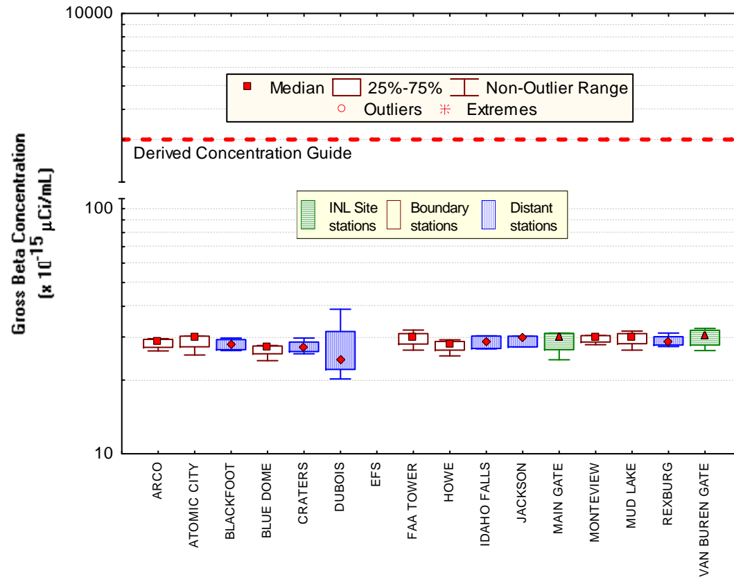
Figure 9. August gross beta concentrations in air at ESER INL Site, Boundary and Distant locations. Number of samples (N) = 4 at each location, except Jackson (N = 3) and EFS (N = 0).
