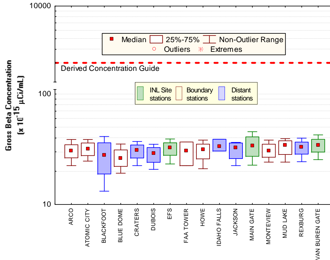
Figure 10. September gross beta concentrations in air at ESER INL Site, Boundary and Distant locations. Number of samples (N) = 4 at each location, except FAA Tower and Idaho Falls (N = 3).
