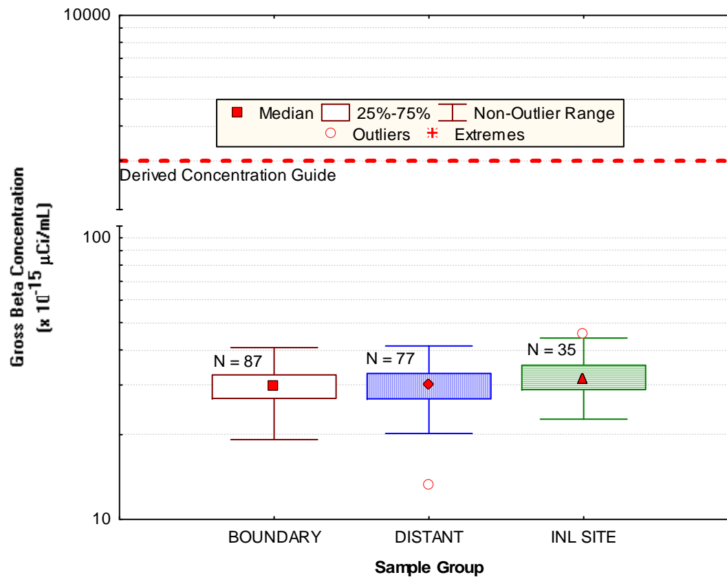
Figure 7. Gross beta concentrations in air at ESER INL Site, Boundary and Distant locations for the third quarter of 2008.
