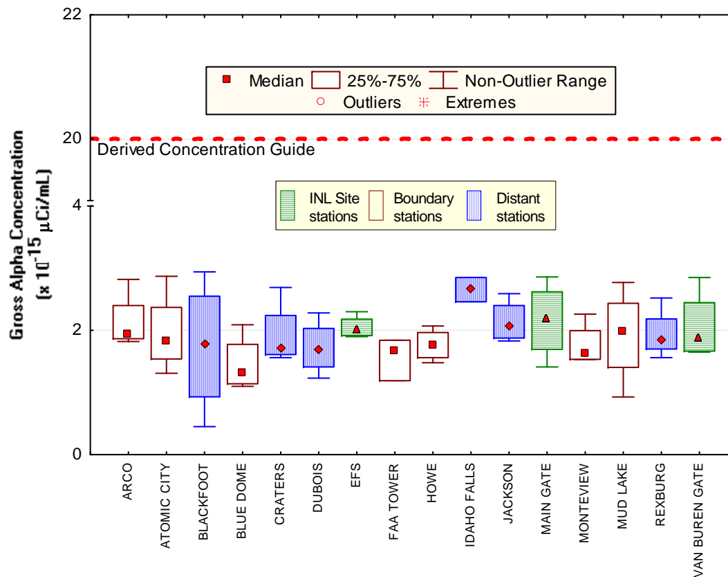
Figure 6. September gross alpha concentrations in air at ESER INL Site, Boundary and Distant locations. Number of samples (N) = 4 at each location, except FAA Tower and Idaho Falls (N = 3).
