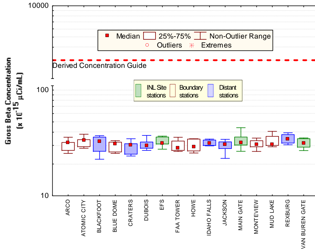
Figure 8. July gross beta concentrations in air at ESER INL Site, Boundary and Distant locations. Number of samples (N) = 5 at each location, except Idaho Falls and Rexburg (N = 4).
