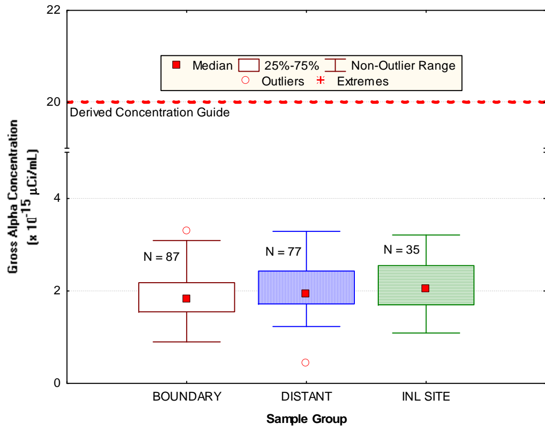
Figure 3. Gross alpha concentrations in air at ESER INL Site, Boundary and Distant locations for the third quarter of 2008.
