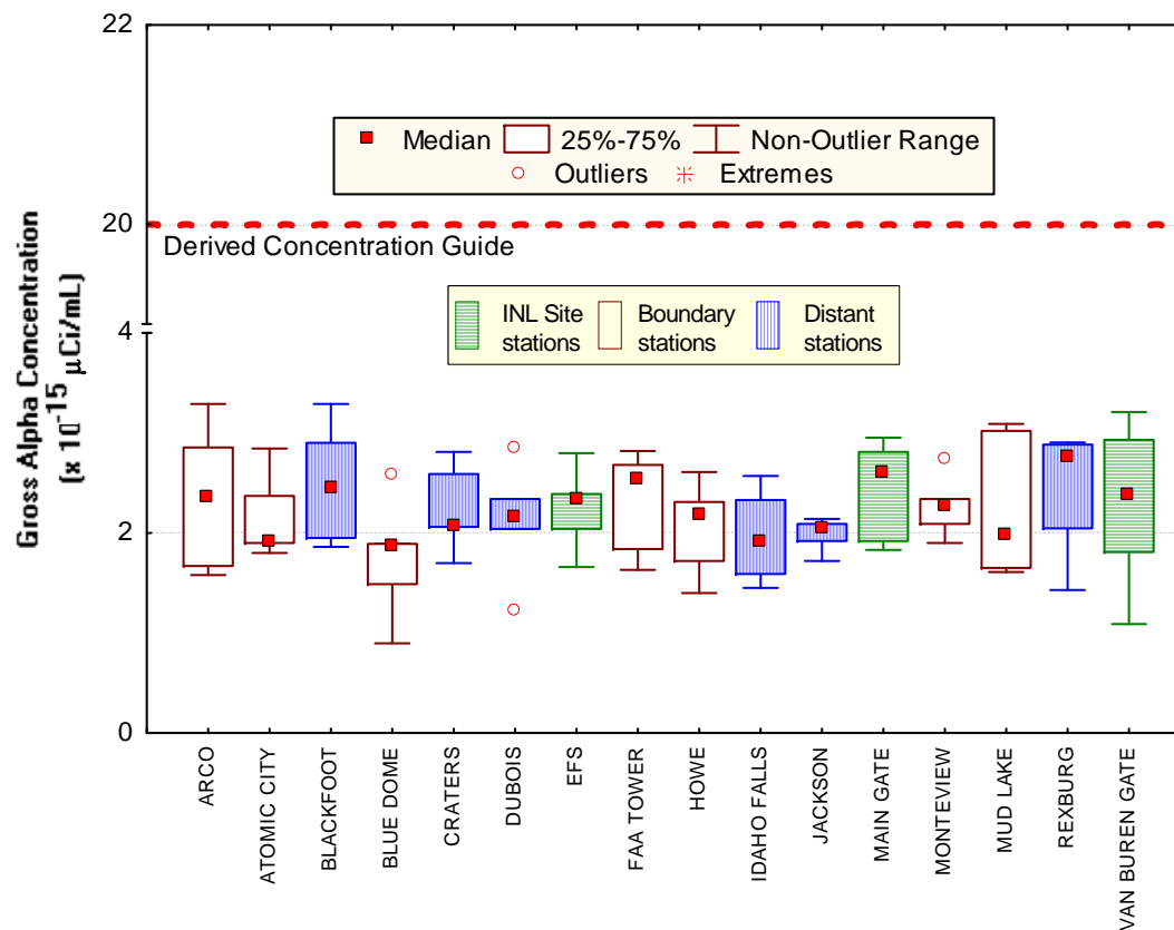
Figure 4. July gross alpha concentrations in air at ESER INL Site, Boundary and Distant locations. Number of samples (N) = 5 at each location, except Idaho Falls and Rexburg (N = 4).
