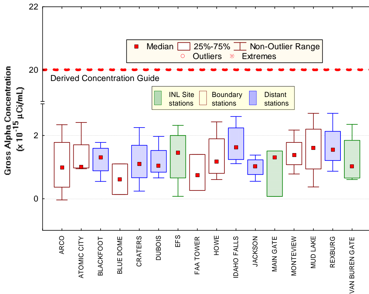
Figure 6. June gross alpha concentrations in air at ESER INL Site, Boundary and Distant locations. Number of samples (N) = 4 at each location, except FAA Tower and Main Gate (N = 3) and Blue Dome (N = 2).
