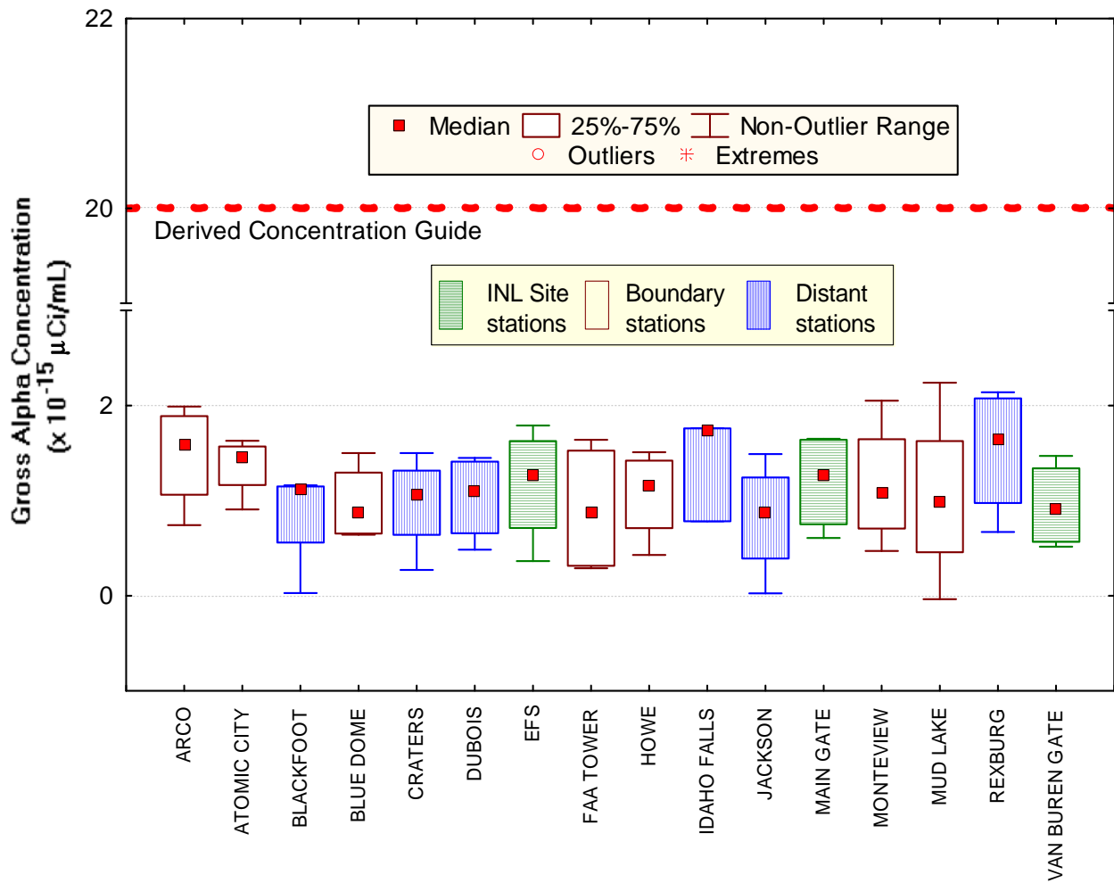
Figure 5. May gross alpha concentrations in air at ESER INL Site, Boundary and Distant locations. Number of samples (N) = 4 at each location, except Idaho Falls (N = 3).
