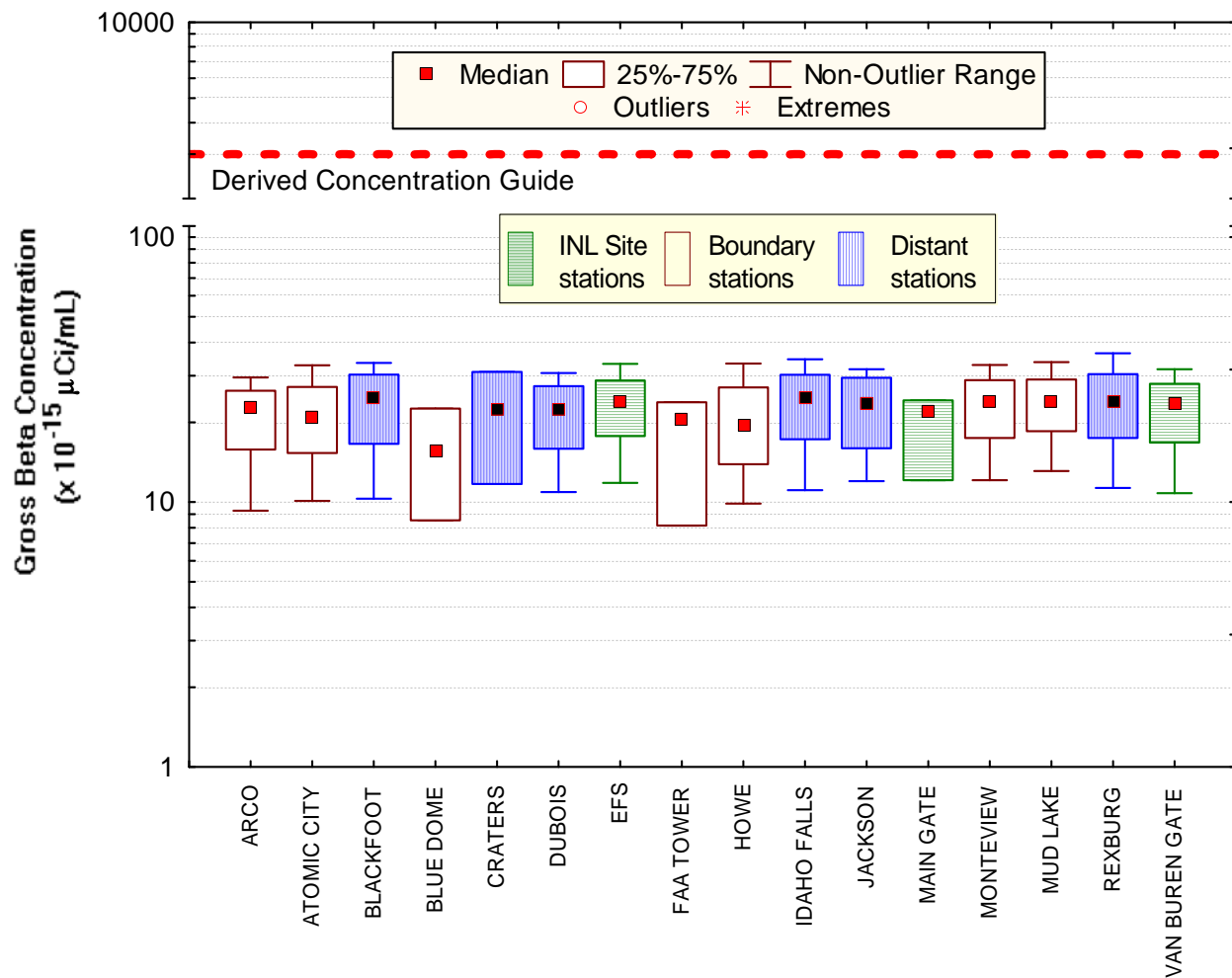
Figure 10. June gross beta concentrations in air at ESER INL Site, Boundary and Distant locations. Number of samples (N) = 4 at each location, except FAA Tower and Main Gate (N = 3) and Blue Dome (N =2).
