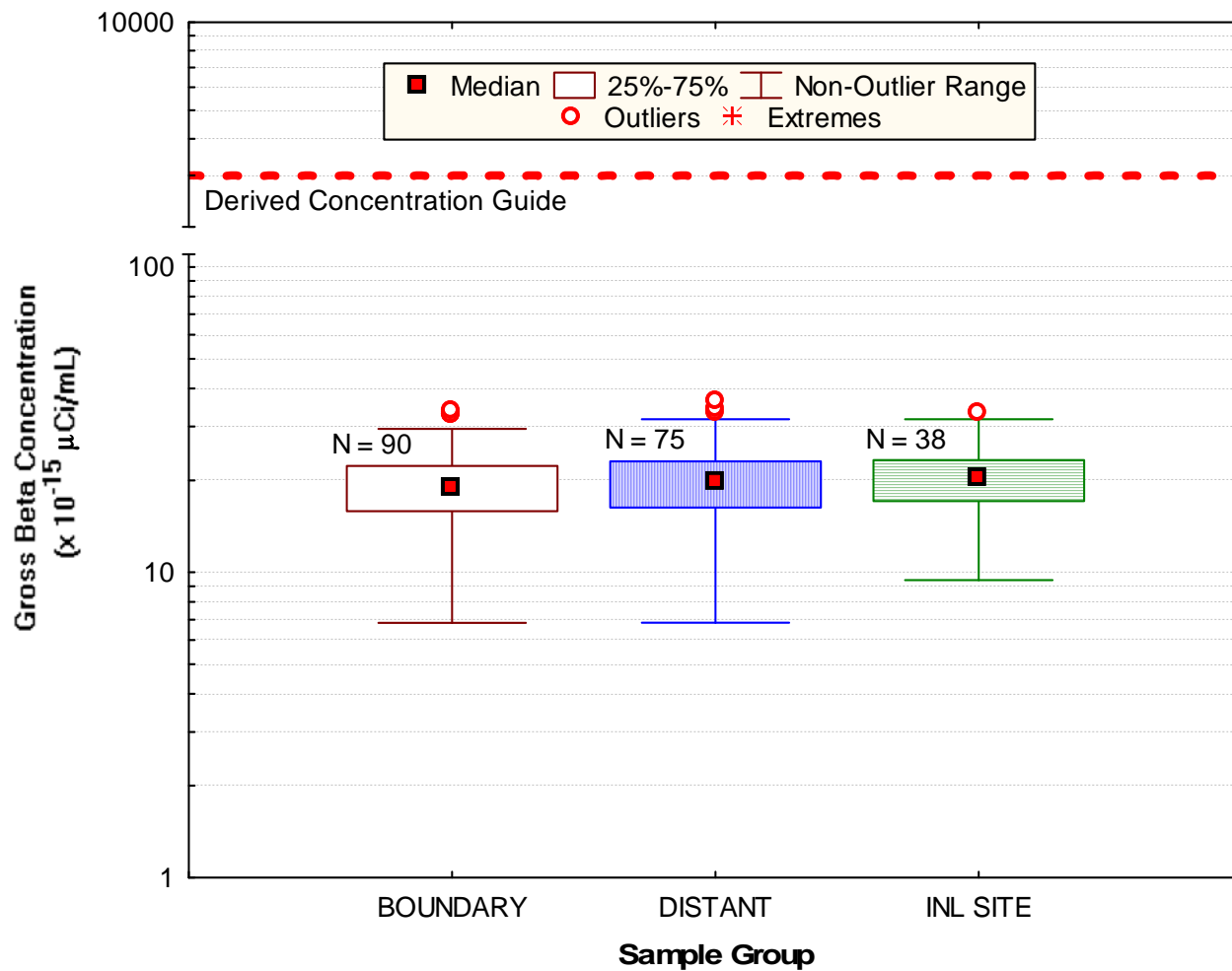
Figure 7. Gross beta concentrations in air at ESER INL Site, Boundary and Distant locations for the second quarter 2008.
