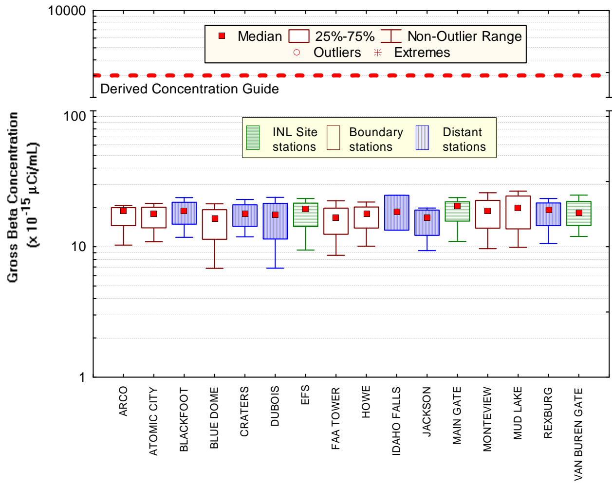
Figure 9. May gross beta concentrations in air at ESER INL Site, Boundary and Distant locations. Number of samples (N) = 4 at each location, except Idaho Falls (N = 3).
