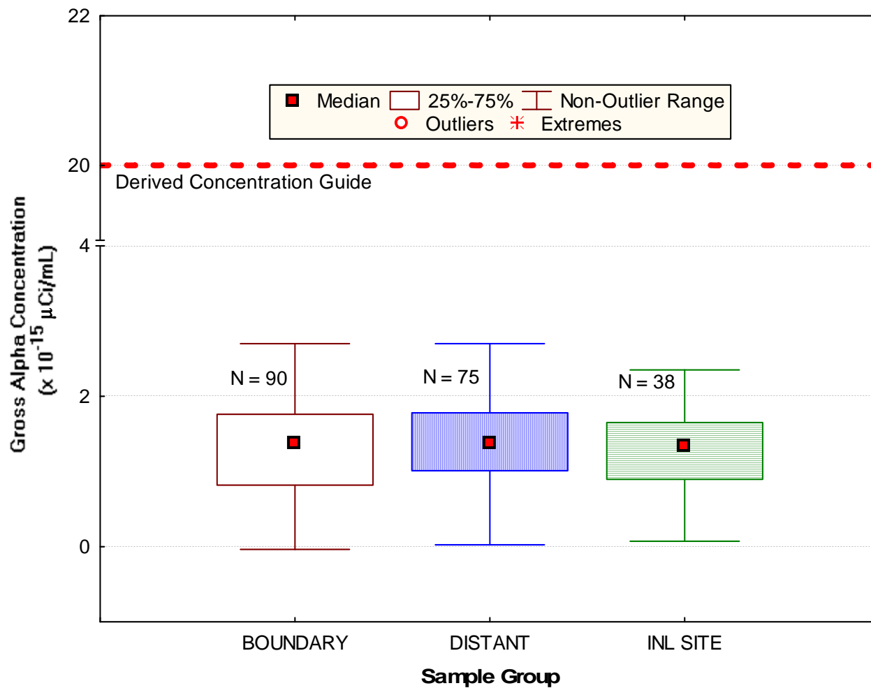
Figure 3. Gross alpha concentrations in air at ESER INL Site, Boundary and Distant locations for the second quarter of 2008.
