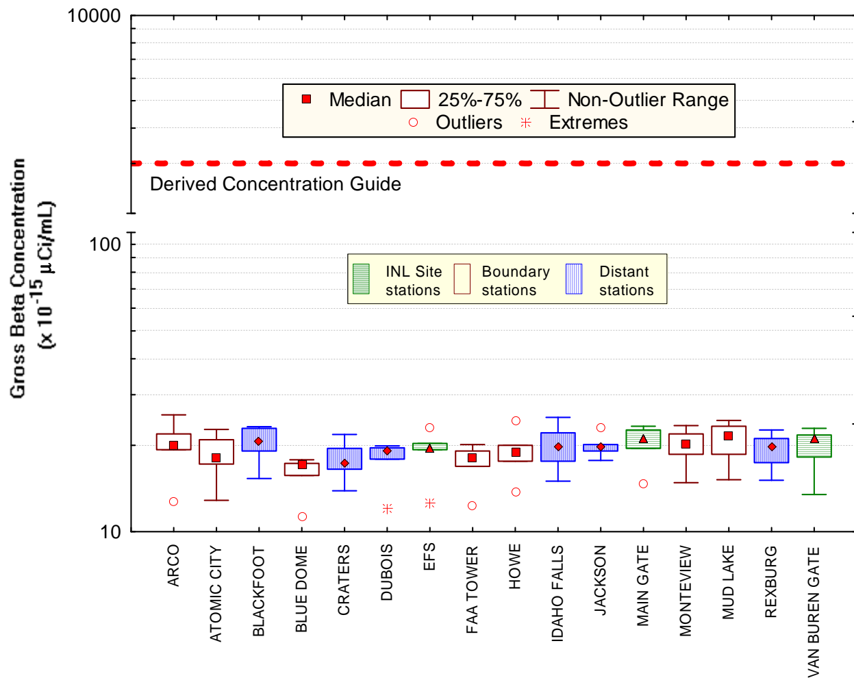
Figure 8. April gross beta concentrations in air at ESER INL Site, Boundary and Distant locations. Number of samples (N) = 5 at each location.
