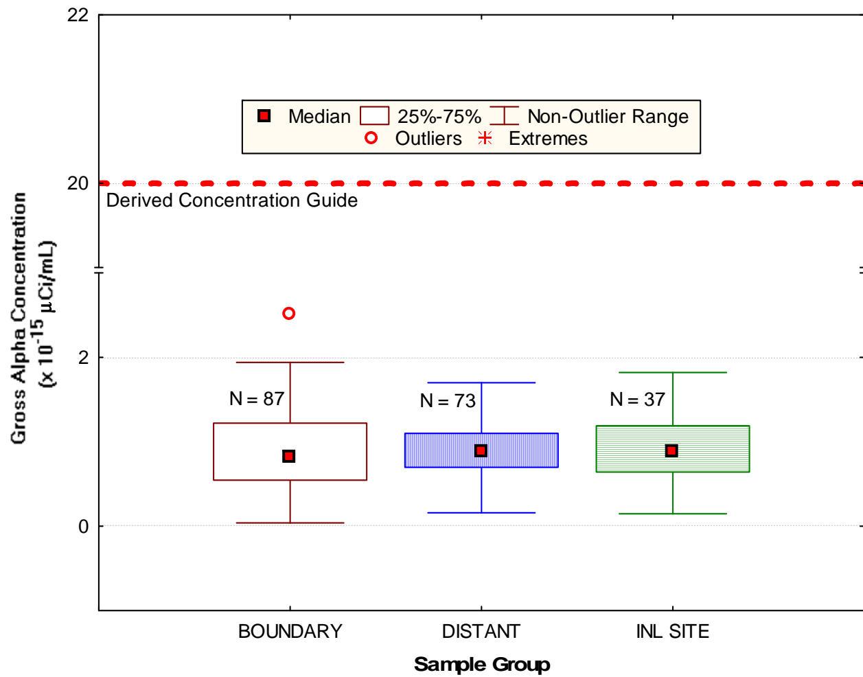
Figure 3. Gross alpha concentrations in air at ESER INL Site, Boundary and Distant locations for the first quarter of 2008.
