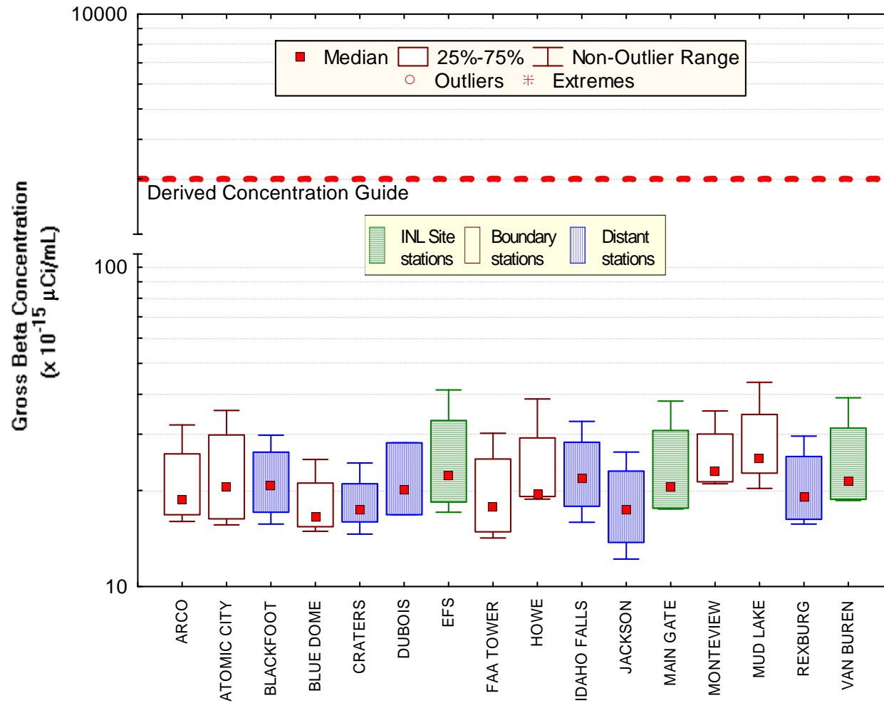
Figure 10. March gross beta concentrations in air at ESER INL Site, Boundary and Distant locations. Number of samples (N) = 4 at each location, except Dubois (N = 3).
