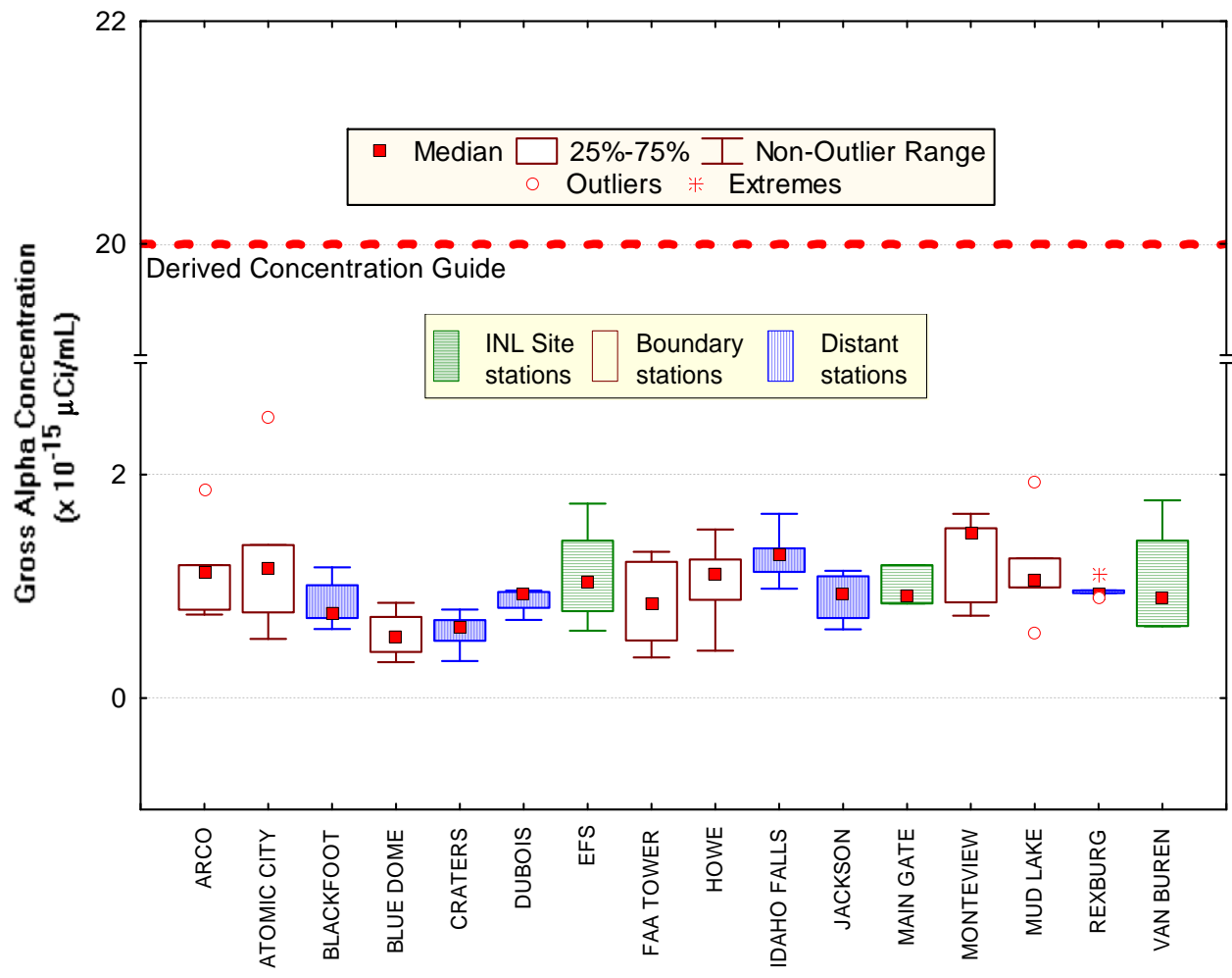
Figure 4. January gross alpha concentrations in air at ESER INL Site, Boundary and Distant locations. Number of samples (N) = 5 at each location, except Blue Dome, Dubois and Jackson (N = 4), and Main Gate (N = 3).
