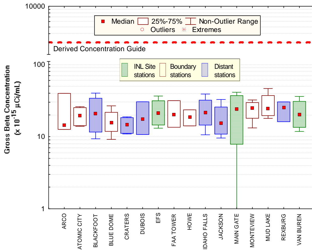
Figure 9. February gross beta concentrations in air at ESER INL Site, Boundary and Distant locations. Number of samples (N) = 4 at each location, except Arco, Dubois, FAA Tower, Howe, and Rexburg (N = 3).
