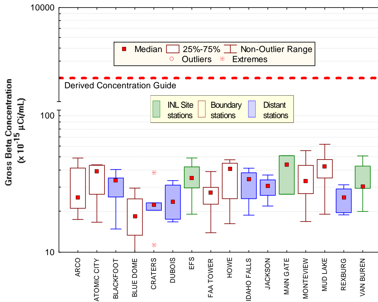
Figure 8. January gross beta concentrations in air at ESER INL Site, Boundary and Distant locations. Number of samples (N) = 5 at each location, except Blue Dome, Dubois and Jackson (N = 4), and Main Gate (N = 3).
