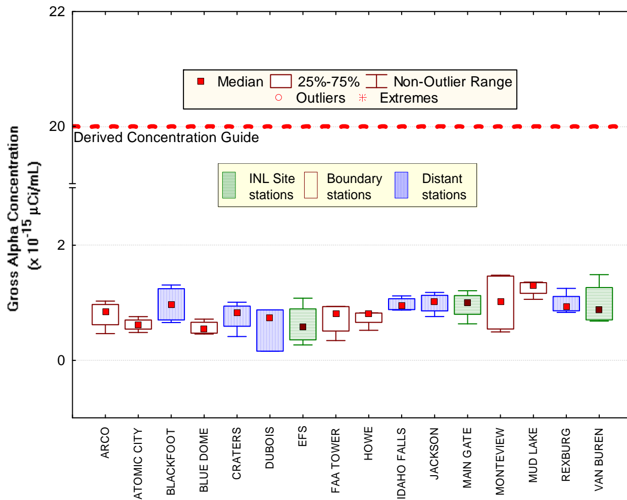
Figure 6. March gross alpha concentrations in air at ESER INL Site, Boundary and Distant locations. Number of samples (N) = 4 at each location, except Dubois (N = 3).
