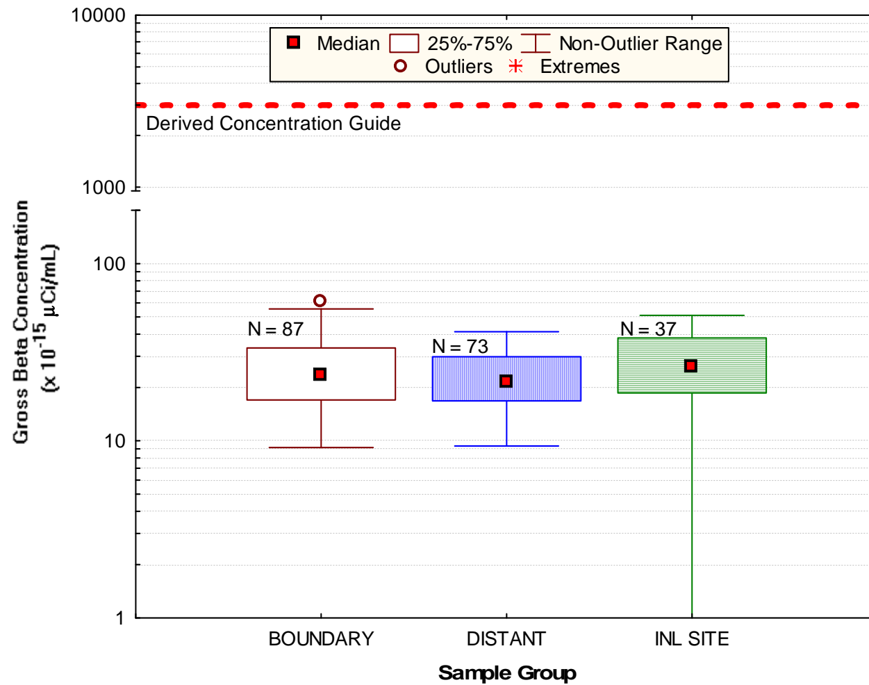
Figure 7. Gross beta concentrations in air at ESER INL Site, Boundary and Distant locations for the first quarter 2008.
