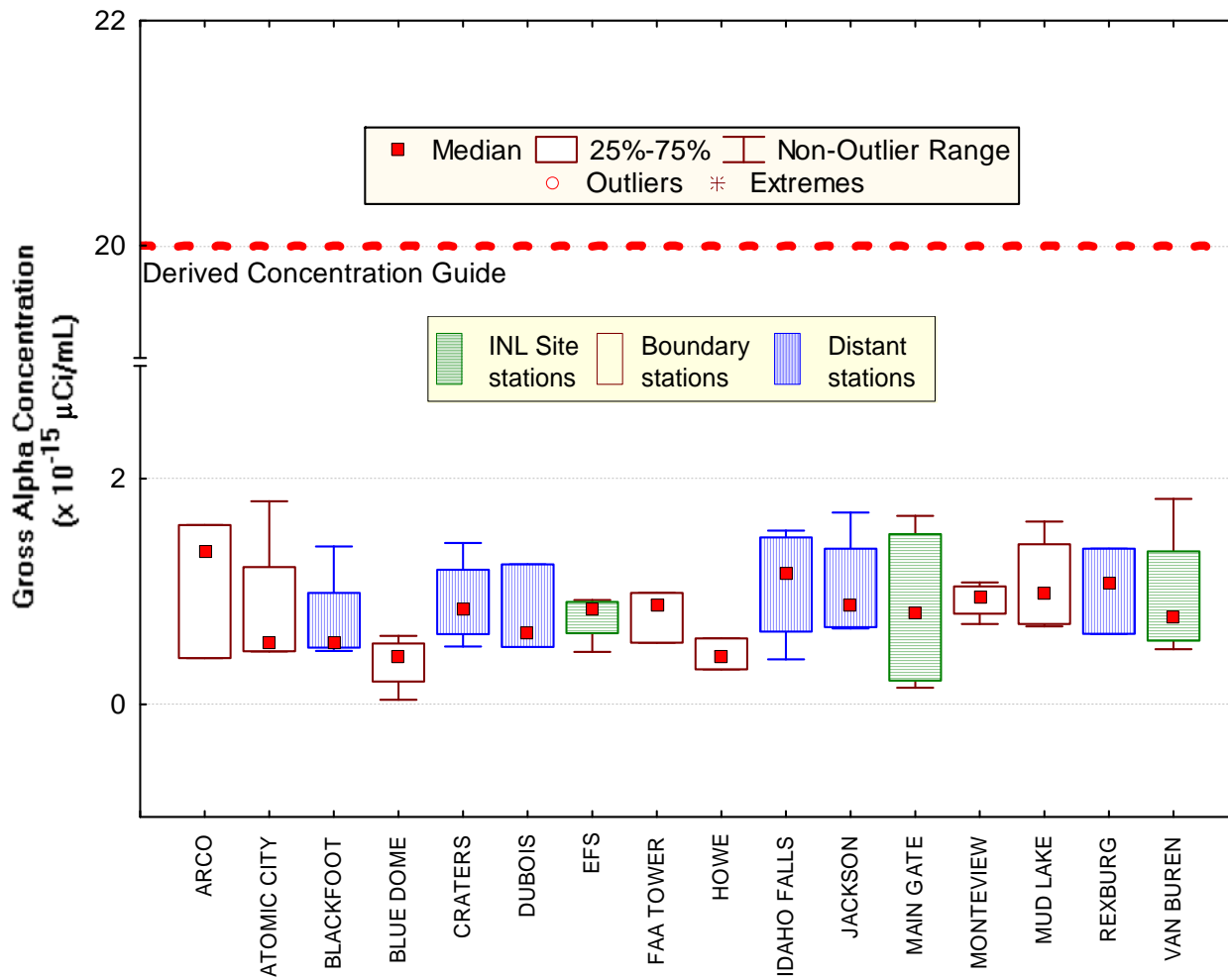
Figure 5. February gross alpha concentrations in air at ESER INL Site, Boundary and Distant locations. Number of samples (N) = 4 at each location, except Arco, Dubois, FAA Tower, Howe, and Rexburg (N = 3).
