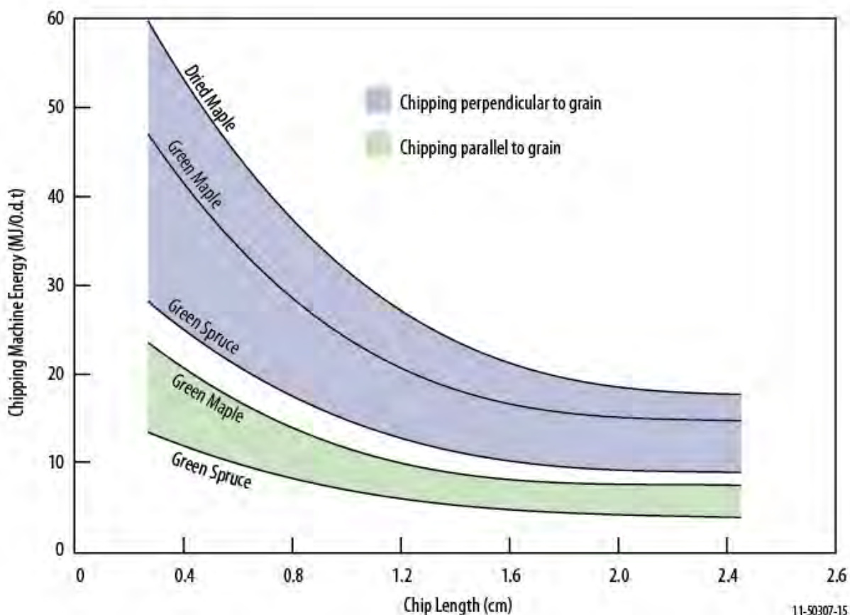
Figure 2-24. The relationship between chip length, cutting angle, and moisture content on energy required for chipping (Pottie and Guimier 1985).
