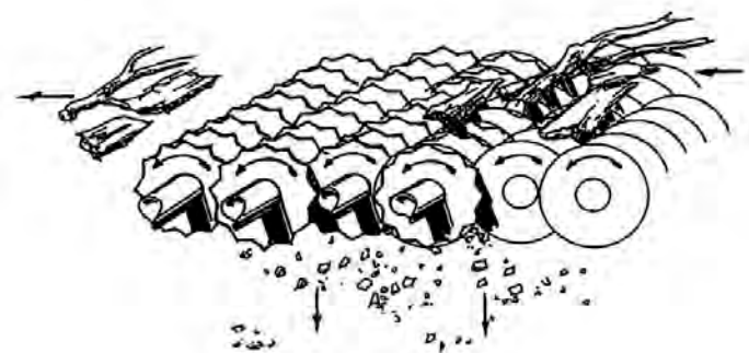
Figure 2-61. Disc screen used to remove overs from a chip stream (Reprinted with permission from Pottie and Guimier 1984).
