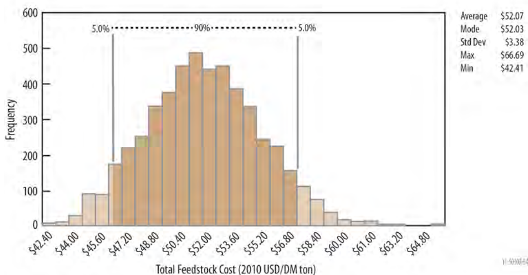
Figure 2-78. Low-Ash/Low-Moisture Conventional woody biomass supply chain cost distribution histogram for pulpwood. Costs are expressed in 2010 $/DM ton.
