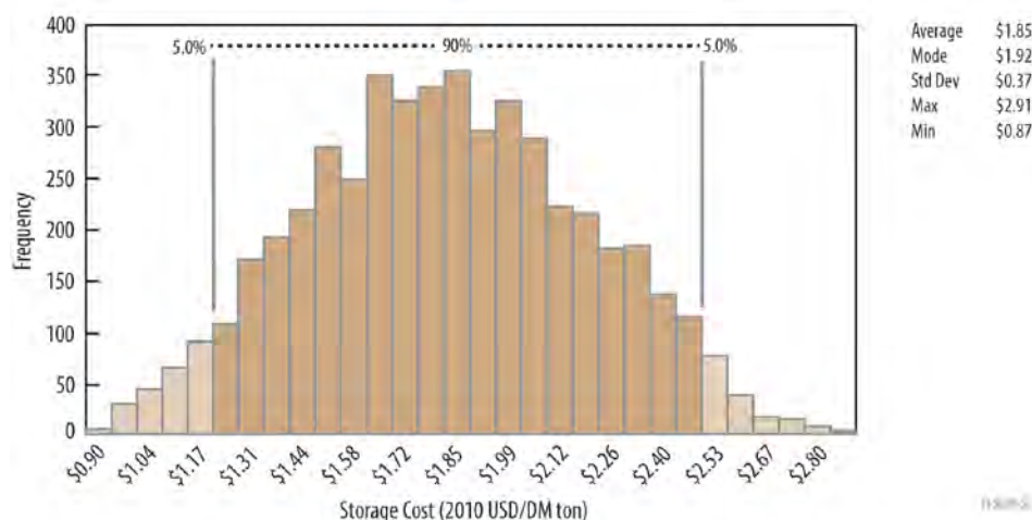
Figure 2-69. Low-Ash/Low-Moisture Conventional woody biomass supply chain cost distribution histogram for the Storage operation for pulpwood. Costs are expressed in 2010 $/DM ton.
