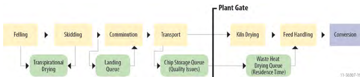
Figure 2-26. Schematic showing an example of hot vs. cold logging systems. The cold logging system, which includes both green circles and yellow boxes, incorporates queuing into the systems.
