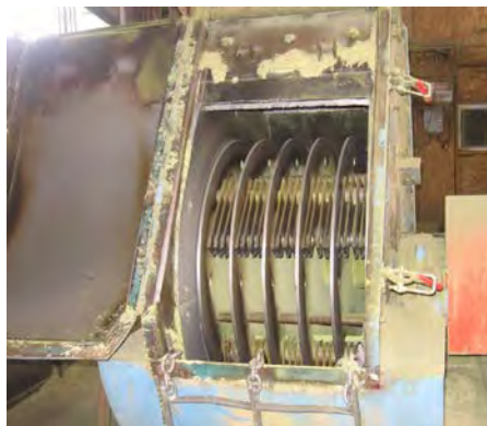
Figure 2-75. Swinging type hammers in an industrial hammer mill.
