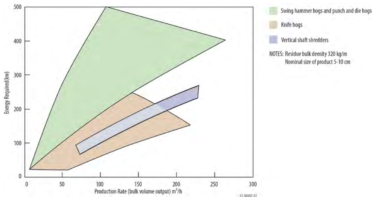
Figure B-6. Energy requirement of various grinder/hog designs (Recreated with permission from Pottie and Guimier 1985).
