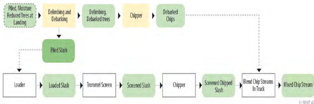
Figure 2-53. Preprocessing supply logistic processes and format intermediates for the Low-Ash/Low-Moisture Conventional design. (Note: Green ovals represent format intermediates and yellow rectangles represent processes modeled in this report. White boxes show alternate designs not modeled in this report).
