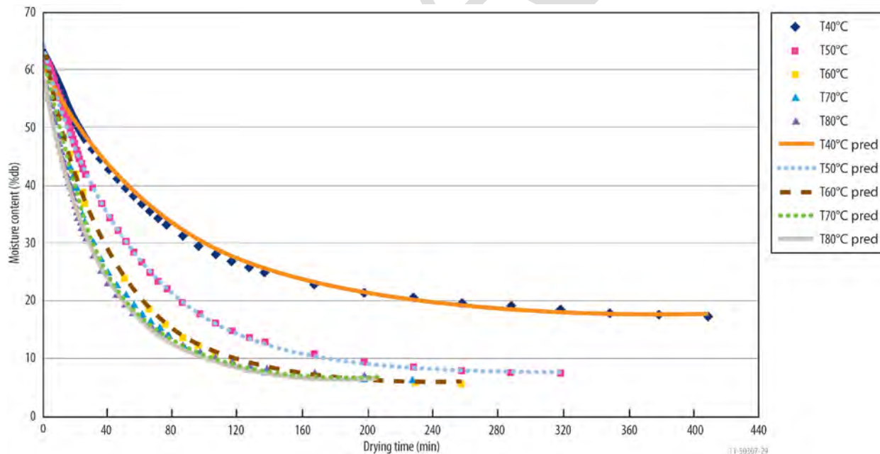
Figure 2-72. Drying rate of forest residues at various drying air temperatures (Phanphanich and Mani 2009). “Pred” indicates predicted values based on drying model produced by Henderson and Pabis (1961).
