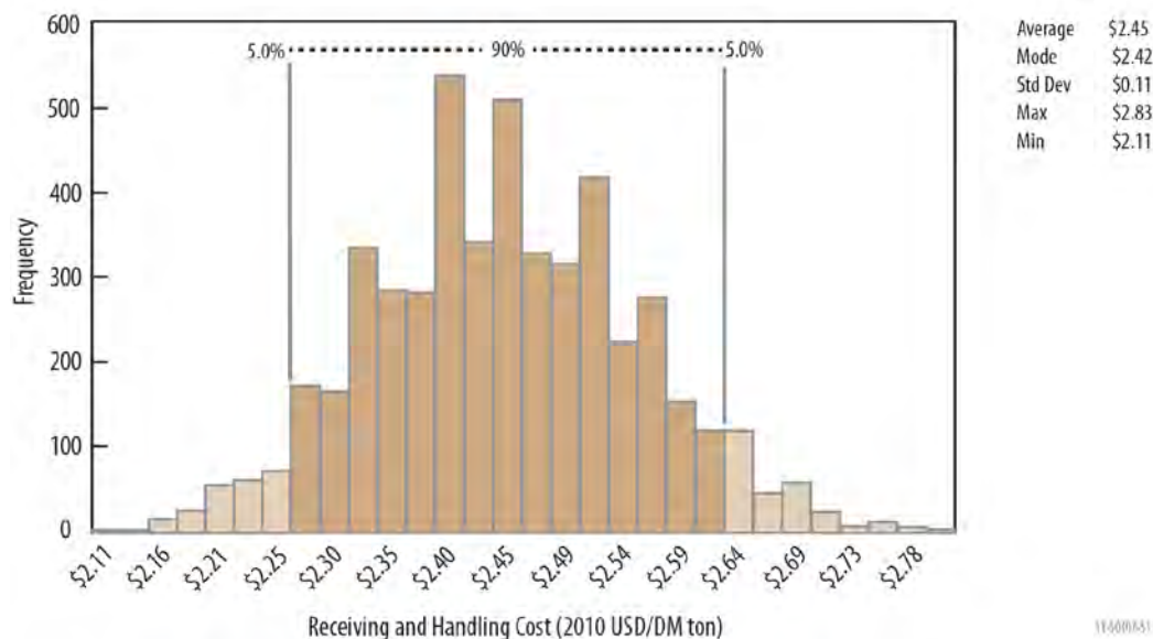
Figure 2-67. Low-Ash/Low-Moisture Conventional woody biomass supply chain cost distribution histogram for the Receiving and Handling operation for pulpwood. Costs are expressed in 2010 $/DM ton.
