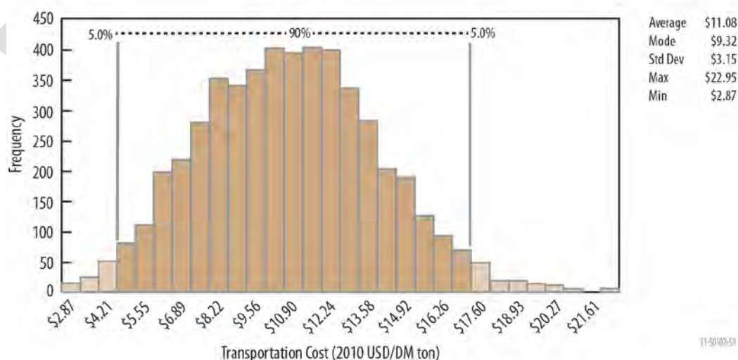
Figure 2-63. Low-Ash/Low-Moisture Conventional woody biomass supply chain cost distribution histogram for the Transportation operation for pulpwood. Costs are expressed in 2010 $/DM ton.
