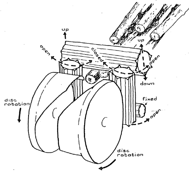
Figure B-4. Schematic of a double-disc chucker (Reprinted with permission from Pottie and Guimier 1984).
