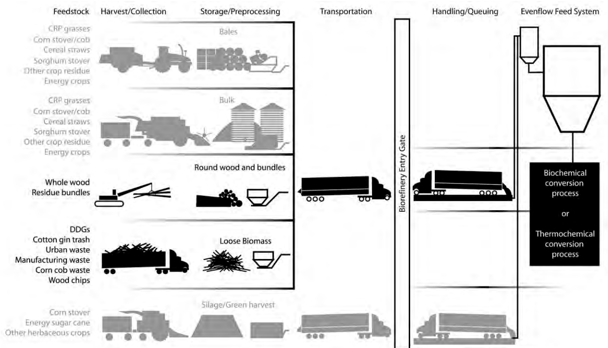
Figure 1-4. Pioneer Uniform-Format feedstock supply system (Pioneer Uniform) designs will allow lignocellulosic biomass to arrive at the biorefinery gate as a uniform-format, flowable material.
