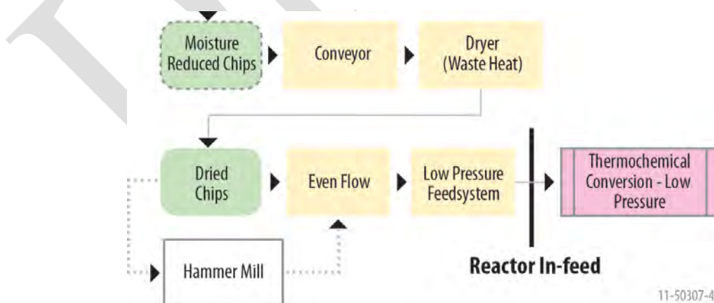
Figure 2-70. In-Plant Handling supply logistic processes and biomass format intermediates for the Low-Ash/Low-Moisture Conventional scenario. (Note: Green ovals represent biomass format intermediates, yellow rectangles represent processes modeled in this report, while white boxes represent processes not modeled. The pink rectangle represents the thermochemical conversion process.)
