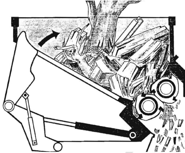
Figure B-3. Schematic of a shredder (Reprinted with permission from Pottie and Guimier 1985).
