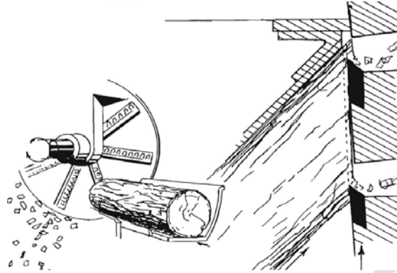
Figure 2-19. Schematic of a disc chipper, similar to that used in the Base Case Conventional design (Pottie and Guimier 1985).
