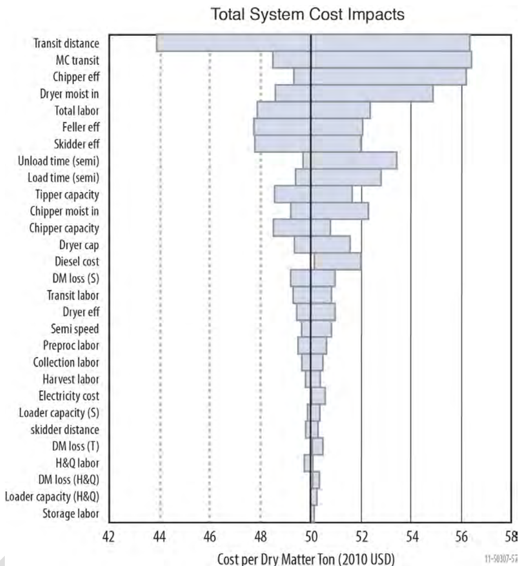
Figure 2-80. Tornado chart reflecting the final cost in dollars according to the distribution ranges defined for the Low-Ash/Low-Moisture Conventional woody biomass feedstock supply system. Costs are expressed in 2010 $/DM ton. Operations are abbreviated by S (Storage), H&Q (Handling and Queuing), and T (Transportation), where applicable.
