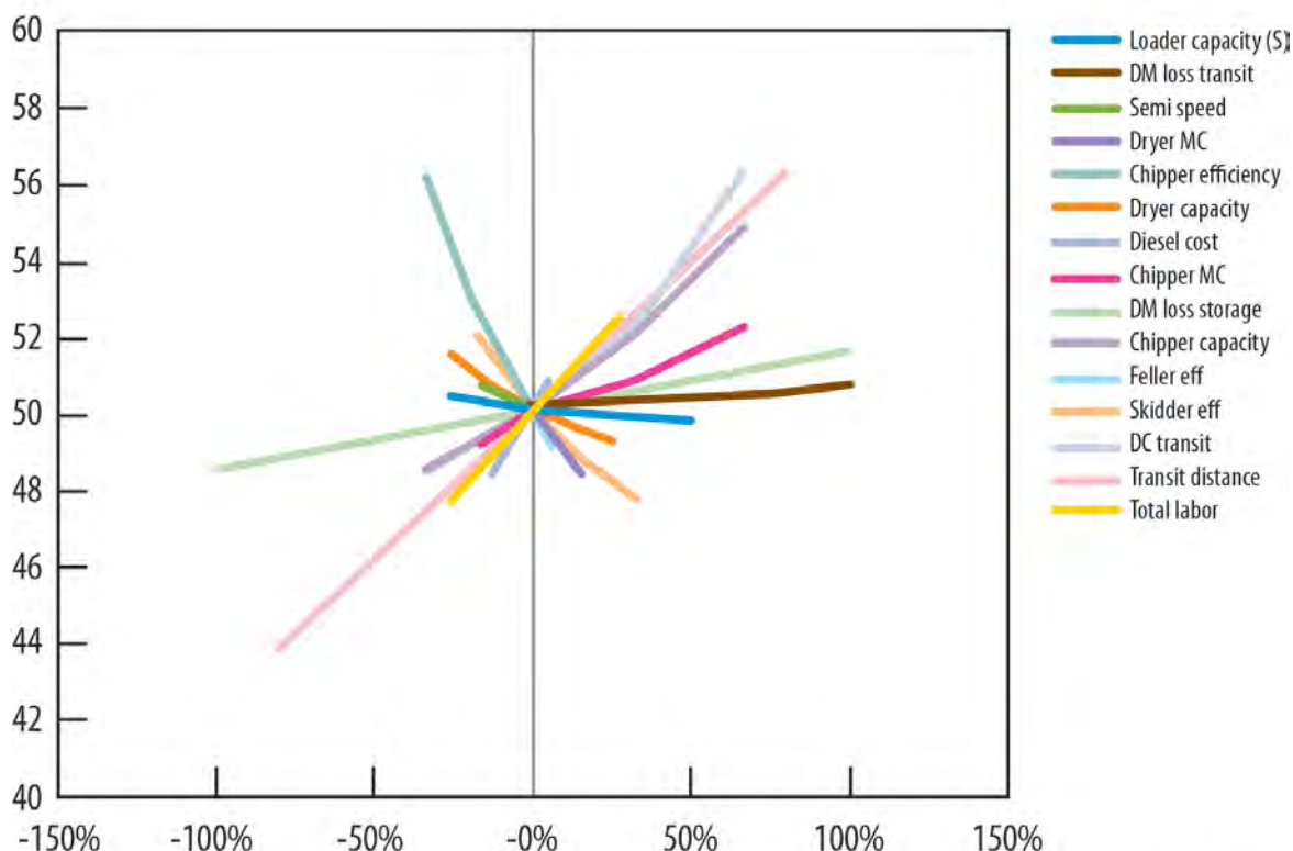
Figure 2-81. Relative impact of various parameters on the cost of supplying biomass through the Low-Ash/Low-Moisture Conventional woody biomass feedstock supply system.
