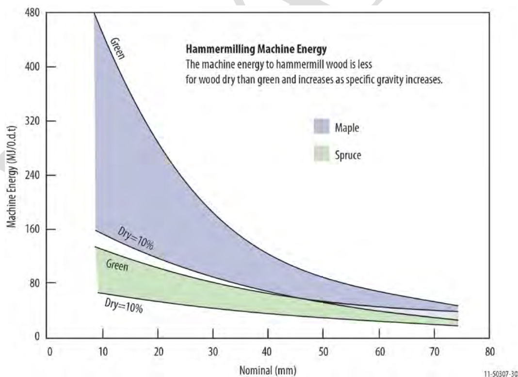
Figure 2-76. Energy consumption during hammer milling of maple and spruce (Recreated with permission from Pottie and Guimier 1985).
