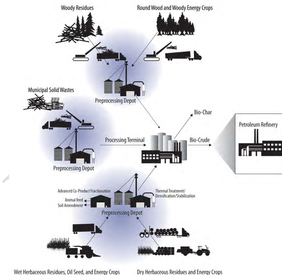
Figure 1-6. Advanced Uniform-Format feedstock supply system designs (Advanced Uniform) follow the model of the current commodity grain supply system, which manages crop diversity at the point of harvest and/or the storage elevator, allowing all subsequent feedstock supply system infrastructure to be similar for all biomass resources.
