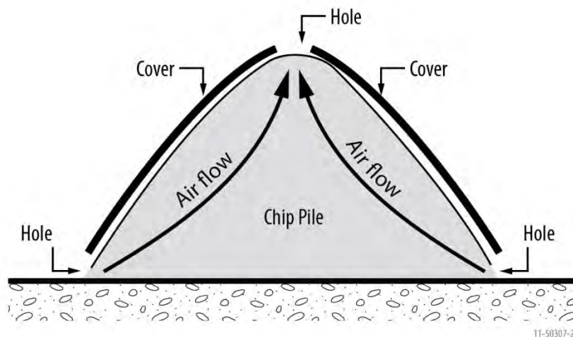
Figure 2-45. Small-scale passive drying method for chips (Recreated with permission from Pottie and Guimier 1985).
