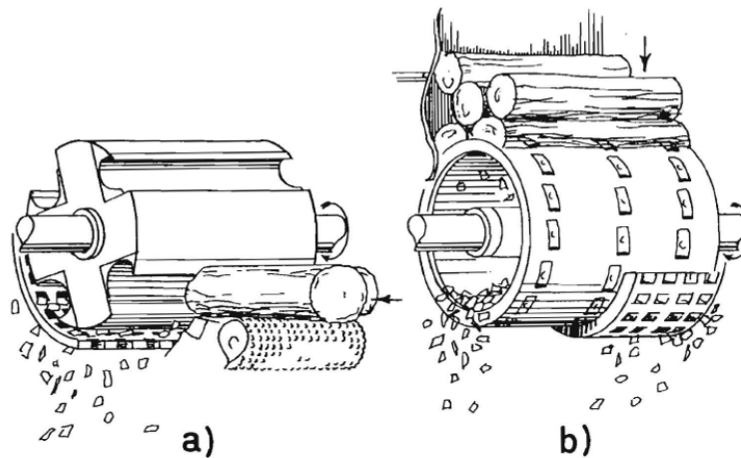
Figure 2-21. Schematic of a drum chipper (Pottie and Guimier 1985). Large knives may be mounted to the drum (a), or smaller knives may be mounted in a spiral pattern around the drum (b).
