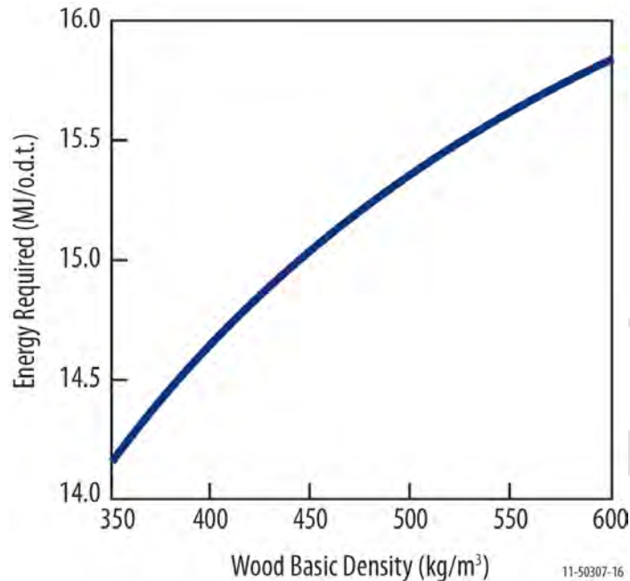
Figure 2-25. Impact of wood density on chipping energy per ton. Chipping energy requirement increases with increasing wood density (Pottie and Guimier 1985).
