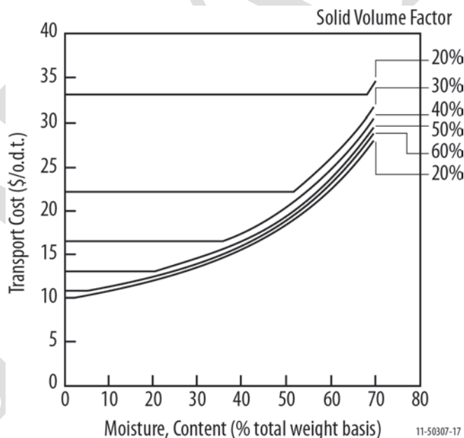
Figure 2-31. Relationship between transportation costs and moisture content considering various solid volume factors. A higher solid volume factor indicates more dense packing (Recreated with permission from Pottie and Guimier 1985).
