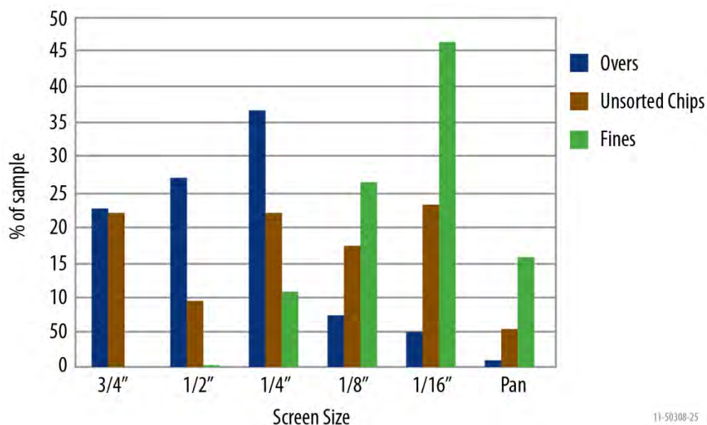
Figure 2-44. Particle size distribution in three piles of comminuted pine trees studied.
