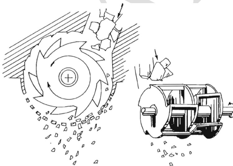
Figure B-2. Schematic of a knife hog (Reprinted with permission from Pottie and Guimier 1985).
