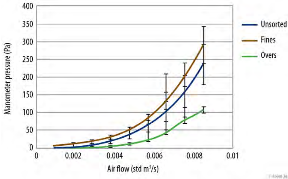
Figure 2-43. Resistance to air flow observed in the three piles studied.
