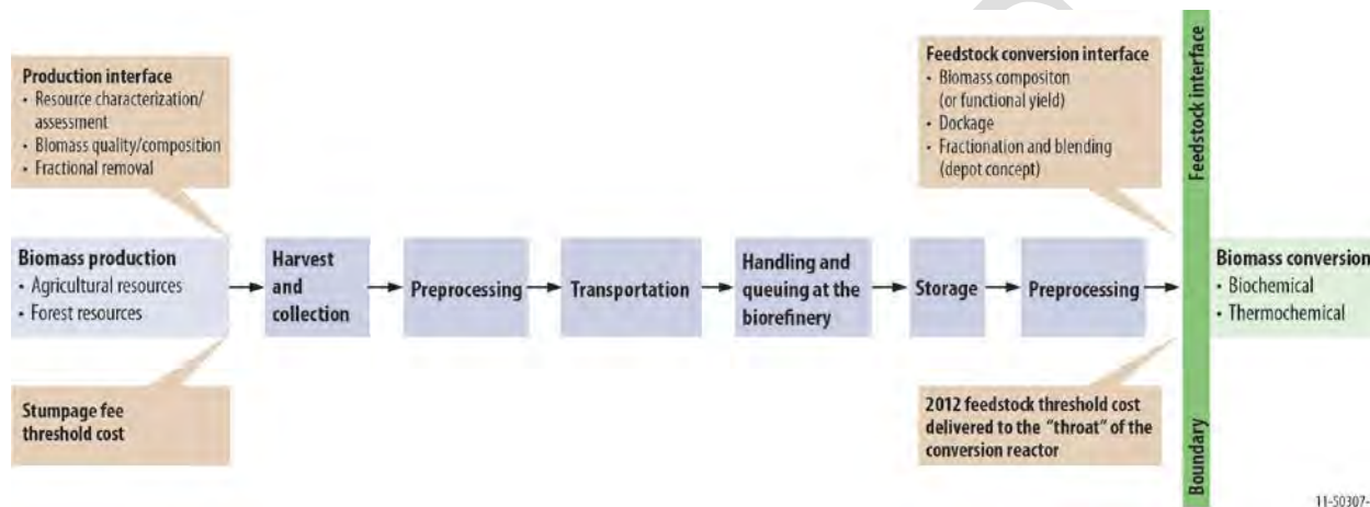
Figure 1-7. Schematic and boundaries for a lignocellulosic feedstock supply system design that allows unit operations to be reordered to achieve optimum supply system performance. Note that the order of operations may change, depending on the supply-chain arrangement.
