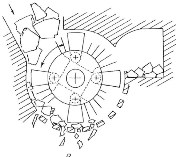
Figure B-1. Schematic of a swing hammer hog (Reprinted with permission from Pottie and Guimier 1985).
