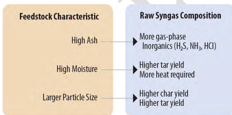
Figure 2-82. Effects of feedstock characteristic on resulting synthesis gas composition out of the gasifier.
