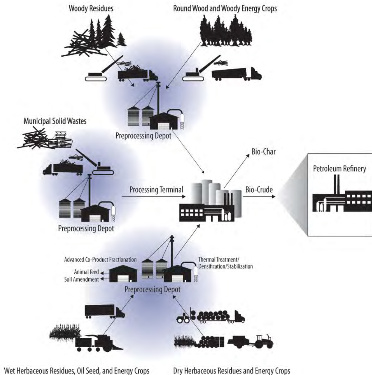
Figure 3-1. The Advanced Uniform-Format feedstock supply system resembles the grain commodity system, which manages crop diversity at the point of harvest and/or the storage elevator, allowing subsequent supply system infrastructure to be similar for all biomass resources.
