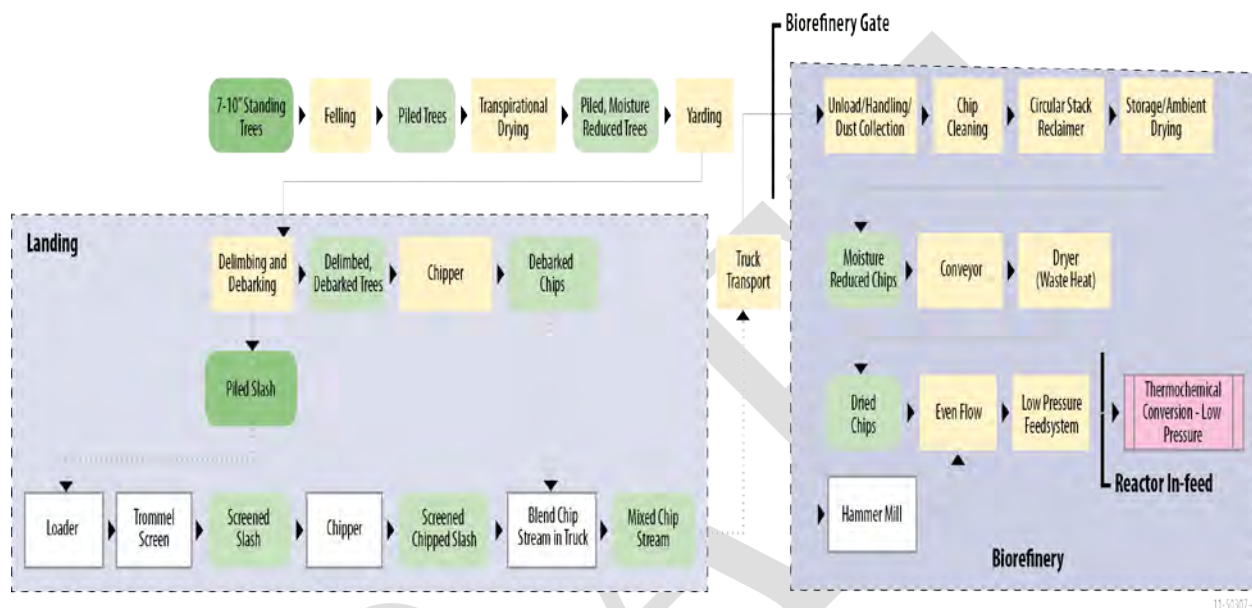
Figure 2-49. Order of unit operations in the Low-Ash/Low-Moisture Conventional feedstock supply system. Operations occurring at the landing and biorefinery are shown in a grey square. (Note: Yellow rectangles represent individual modeled processes, green ovals represent changes in format intermediates, and white rectangles represent alternate processes that were not modeled.)
