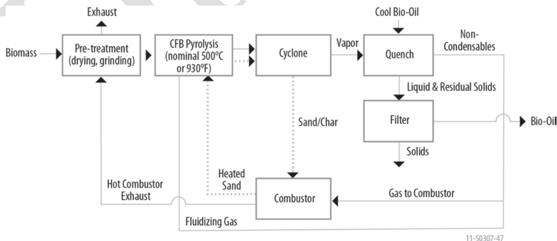
Figure 2-84. An example flowsheet for a circulating fluid bed system for fast pyrolysis.
