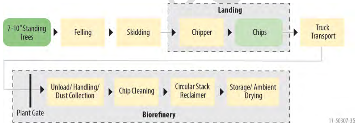
Figure 2-1. Order of unit operations in the Base Case Conventional Woody feedstock supply system design. Operations occurring at the landing are shown in the upper gray square, while operations occurring at the biorefinery are shown in the lower gray square. Note: Yellow rectangles represent individual modeled processes, while green ovals represent changes in format intermediates.)
