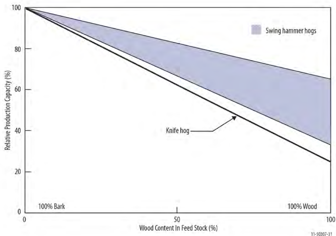
Figure B-5. Impact of changing wood and bark content on production capacity of various grinders (Recreated with permission from Pottie and Guimier 1985). Capacity increases while grinding a higher percentage of bark, and swing-hammer hogs have a higher capacity than knife hogs.
