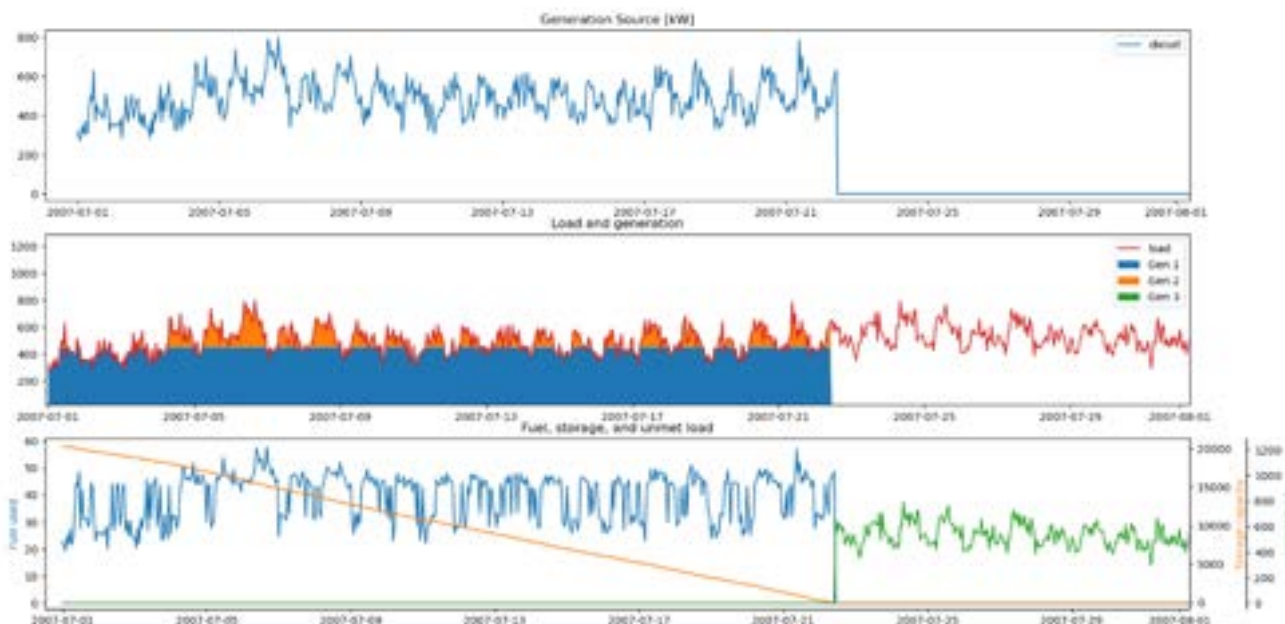
Figure 11. No wind, Year 2, missed fuel shipment (Culler et al. 2022b)
