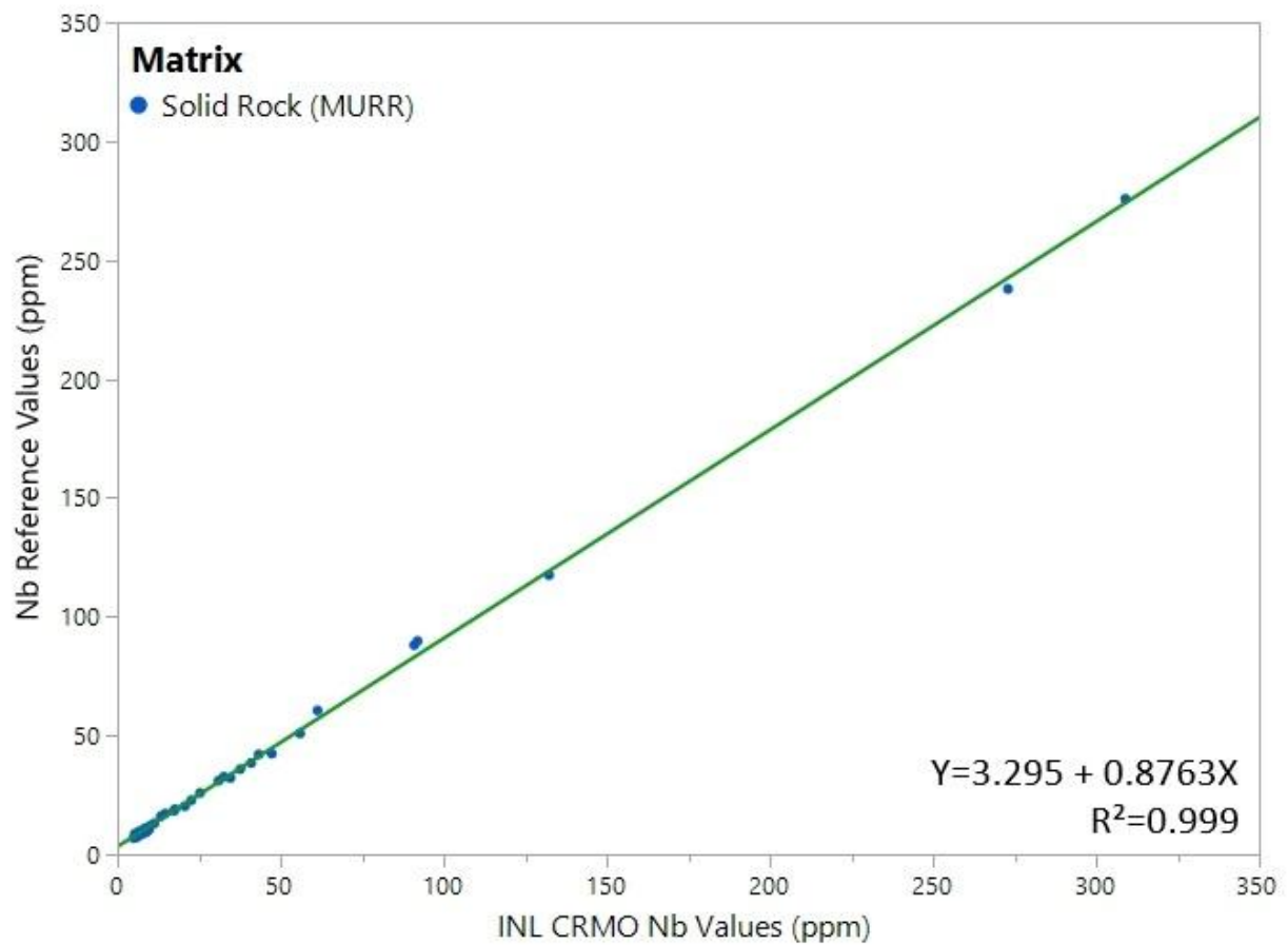
Figure 16. FP calibrated Nb values (in ppm) vs. published reference values. The calibration curve for Nb is shown in green.
