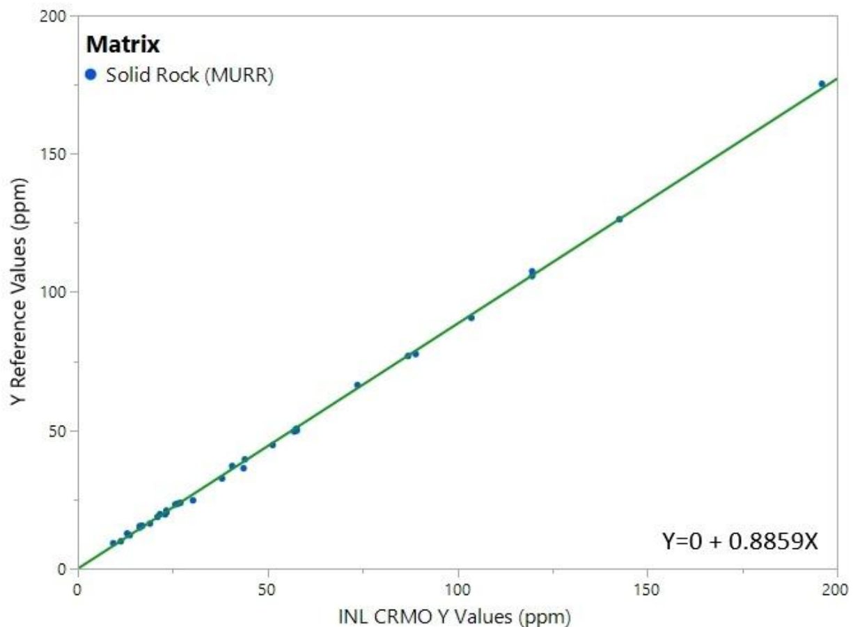
Figure 14. FP calibrated Y values (in ppm) vs. published reference values. The calibration curve for Y is shown in green.
