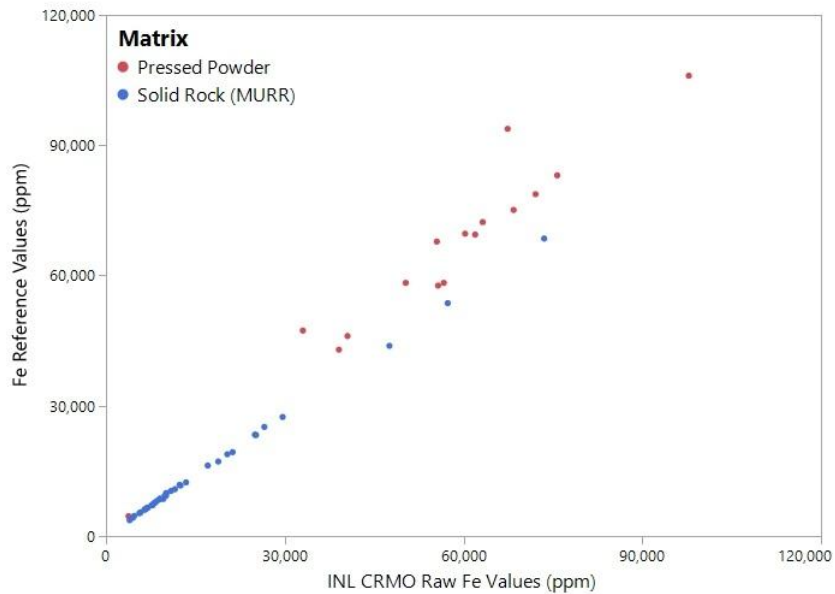
Figure 8. Bi-plot of FP calibrated Fe values (in ppm) vs. published reference values.
