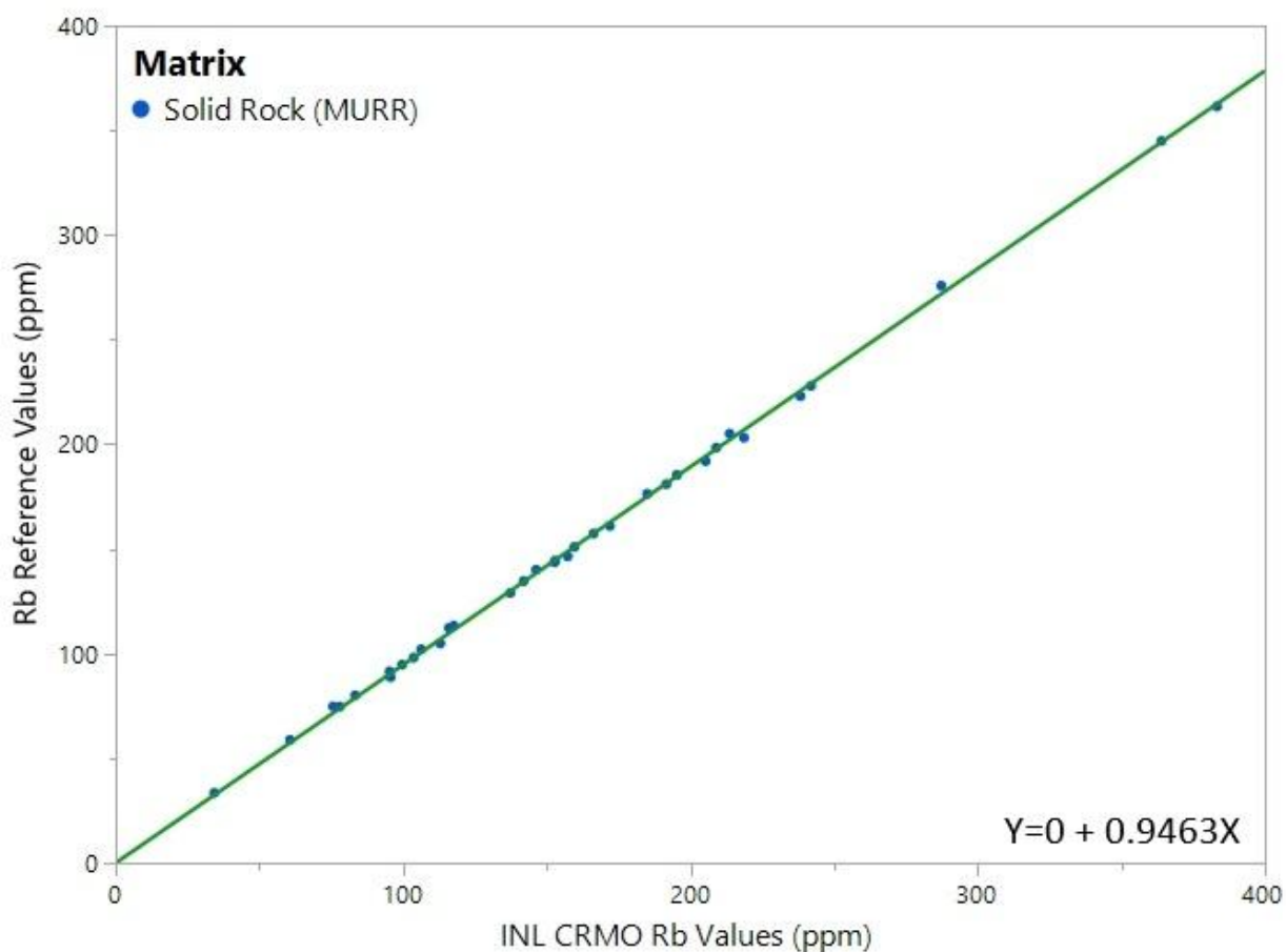
Figure 11. FP calibrated Rb values (in ppm) vs. published reference values. The calibration curve for Rb is shown in green.
