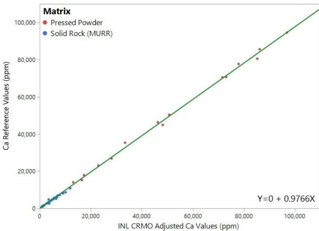
Figure 4. LE adjusted Ca values (in ppm) vs. published reference values. The calibration curve for Ca is shown in green.
