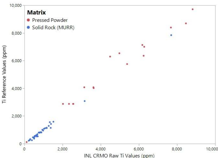
Figure 5. Bi-plot of FP calibrated Ti values (in ppm) vs. published reference values.
