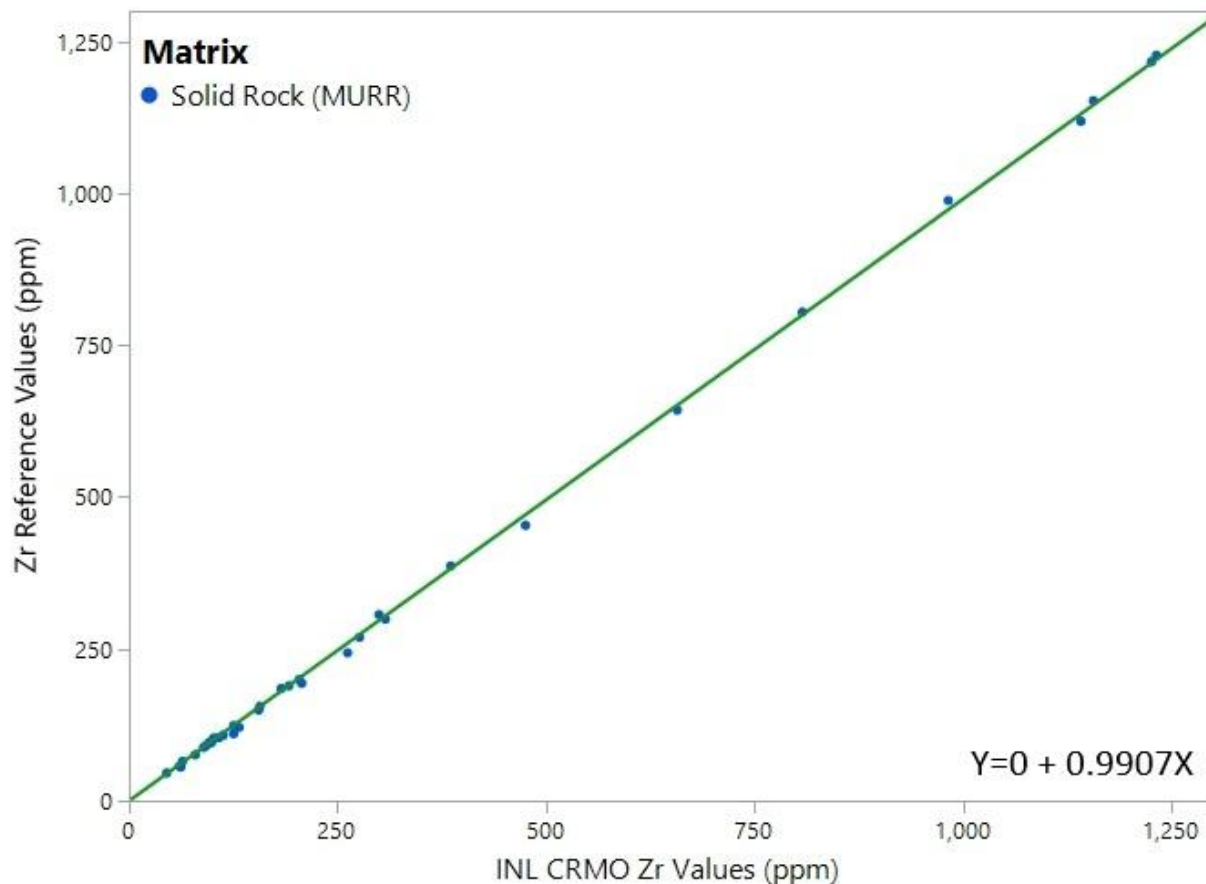
Figure 15. FP calibrated Zr values (in ppm) vs. published reference values. The calibration curve for Zr is shown in green.
