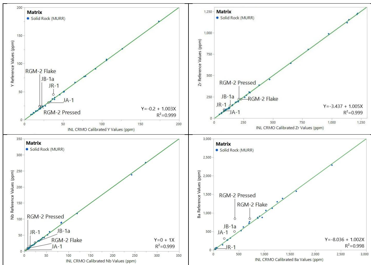
Figure 18. Calibration validation showing calibrated elemental values (in ppm) vs. published reference values with associated regression lines. The reference standards used to validate the accuracy of the calibration are labeled.
