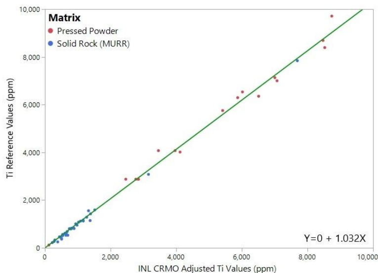
Figure 6. LE adjusted Ti values (in ppm) vs. published reference values. The calibration curve for Ti is shown in green.
