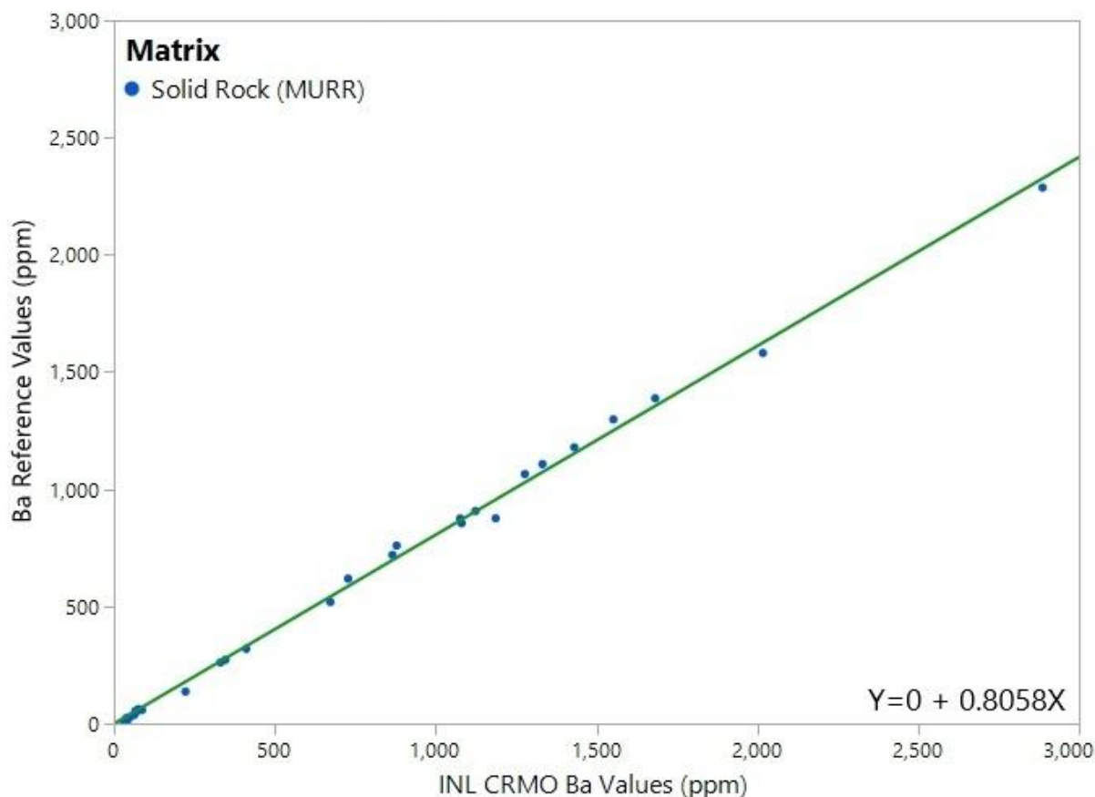
Figure 17. FP calibrated Ba values (in ppm) vs. published reference values. The calibration curve for Ba is shown in green.
