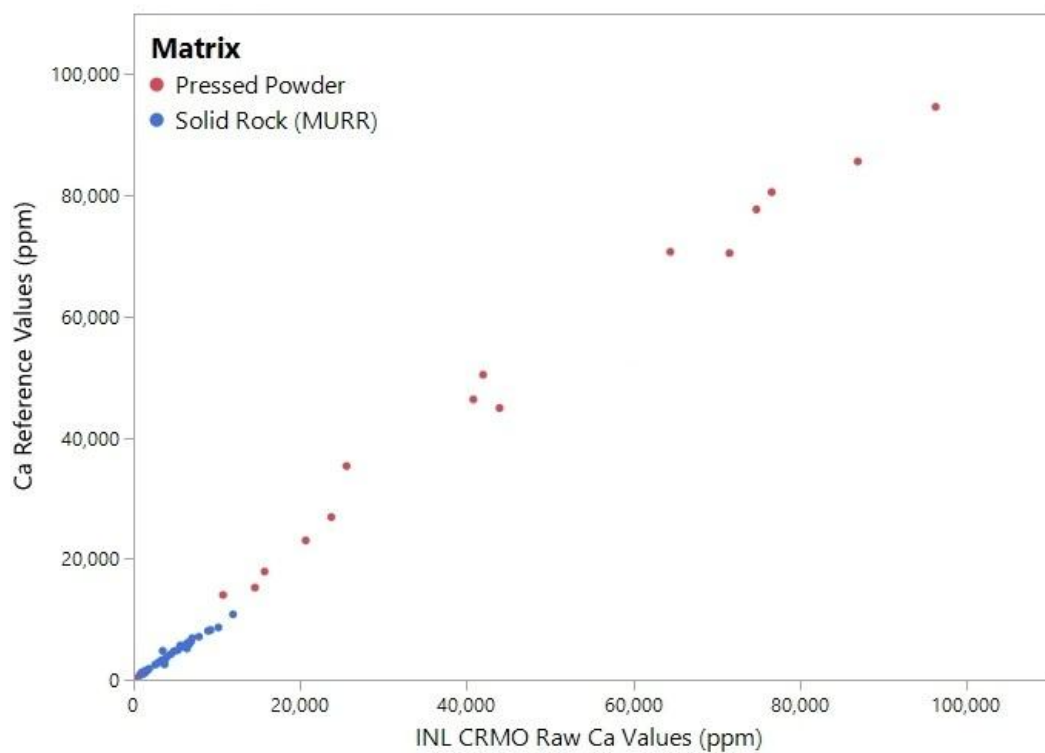
Figure 3. Bi-plot of FP calibrated Ca values (in ppm) vs. published reference values.
