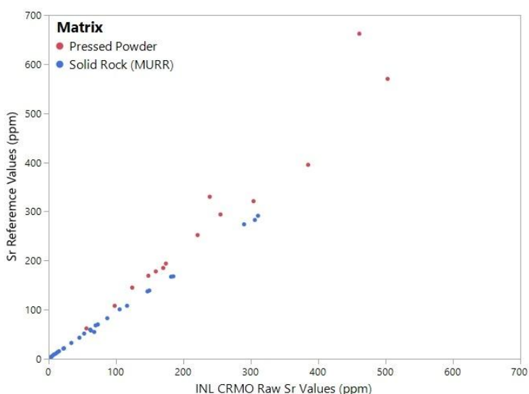
Figure 12. Bi-plot of FP calibrated Sr values (in ppm) vs. published reference values.
