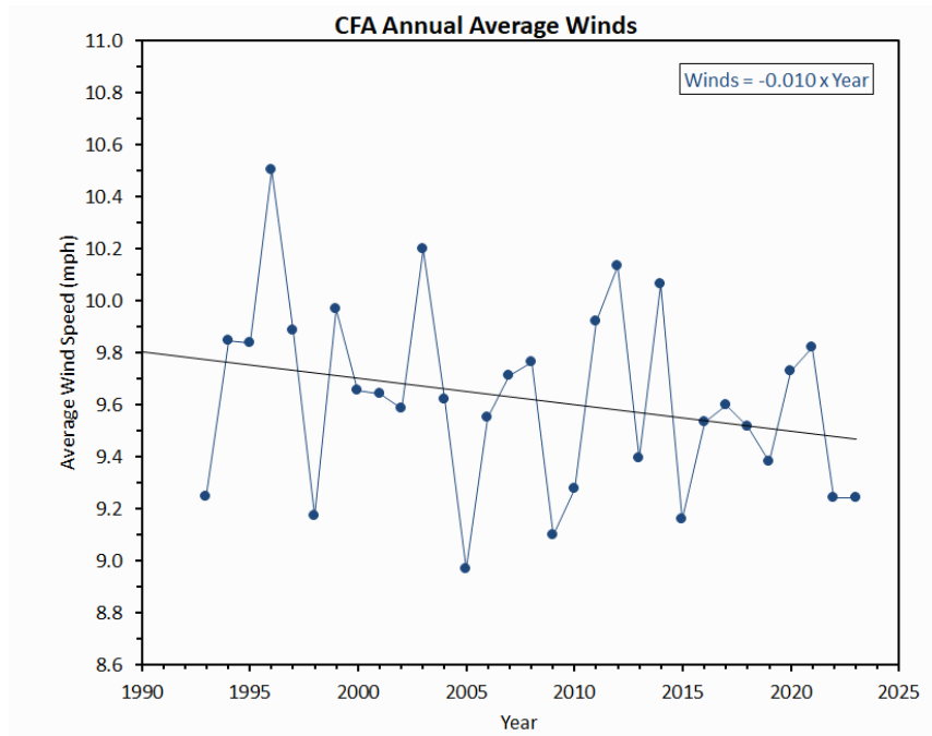
Figure 10. Mean annual wind speed data for CFA using five-minute wind speed data totals averaged for each year of record at CFA from 1993 through 2023. The linear trend line and regression slope are also shown.
