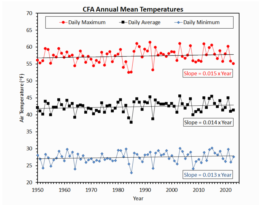
Figure 6. Mean air temperature for INL Site using daily maximum (dot), daily average (square), or daily minimum (diamond) temperatures from 1950 through 2023. Linear trend lines and the linear regression slopes are also shown.
