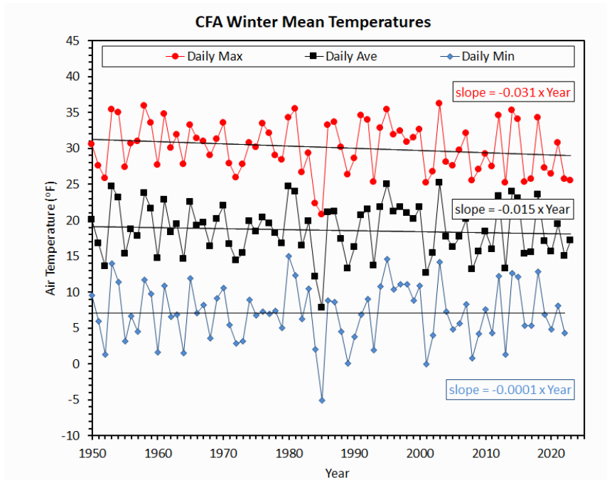
Figure 7. Winter season mean air temperature for CFA using daily maximum (dot), daily average (square), or daily minimum (diamond) temperatures from 1950 through 2023. Linear trend lines and the regression slopes are also shown. The year on the plot represents the year the winter season started.
