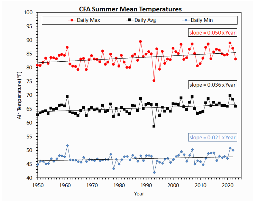
Figure 8. Summer season mean air temperature for CFA using daily maximum (dot), daily average (square), or daily minimum (diamond) temperatures from 1950 through 2023. Linear trend lines and the regression slopes are also shown.
