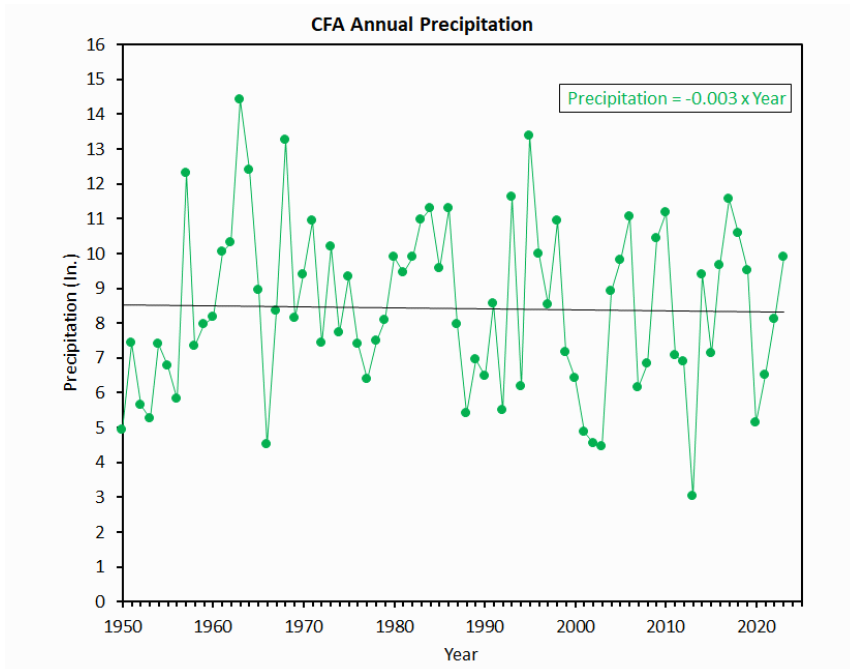
Figure 9. Mean annual precipitation for CFA using daily precipitation totals averaged for each year of record at CFA from 1950 through 2023. The linear trend line and regression slope are also shown.
